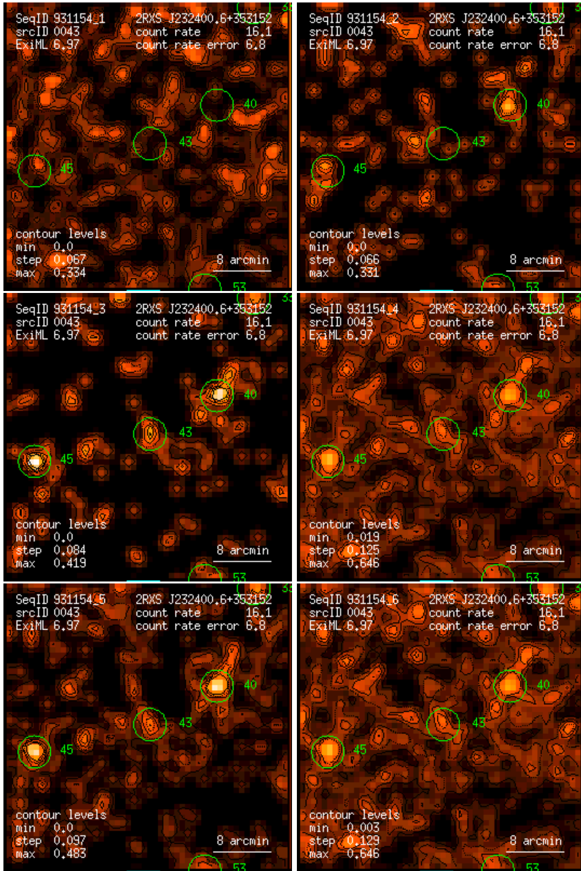
Figure 43: RASS 931154: detection 0043: band rate images, Gaussian filter: (1) PSPC channels 11 – 41, (2) 52 – 90, (3) 91 – 201, (4) 11 – 235, (5) 52 – 201, (6) 11 – 201. Broad band rates in counts/ks. Band rate contour levels in counts/ks/arcmin 2 .
