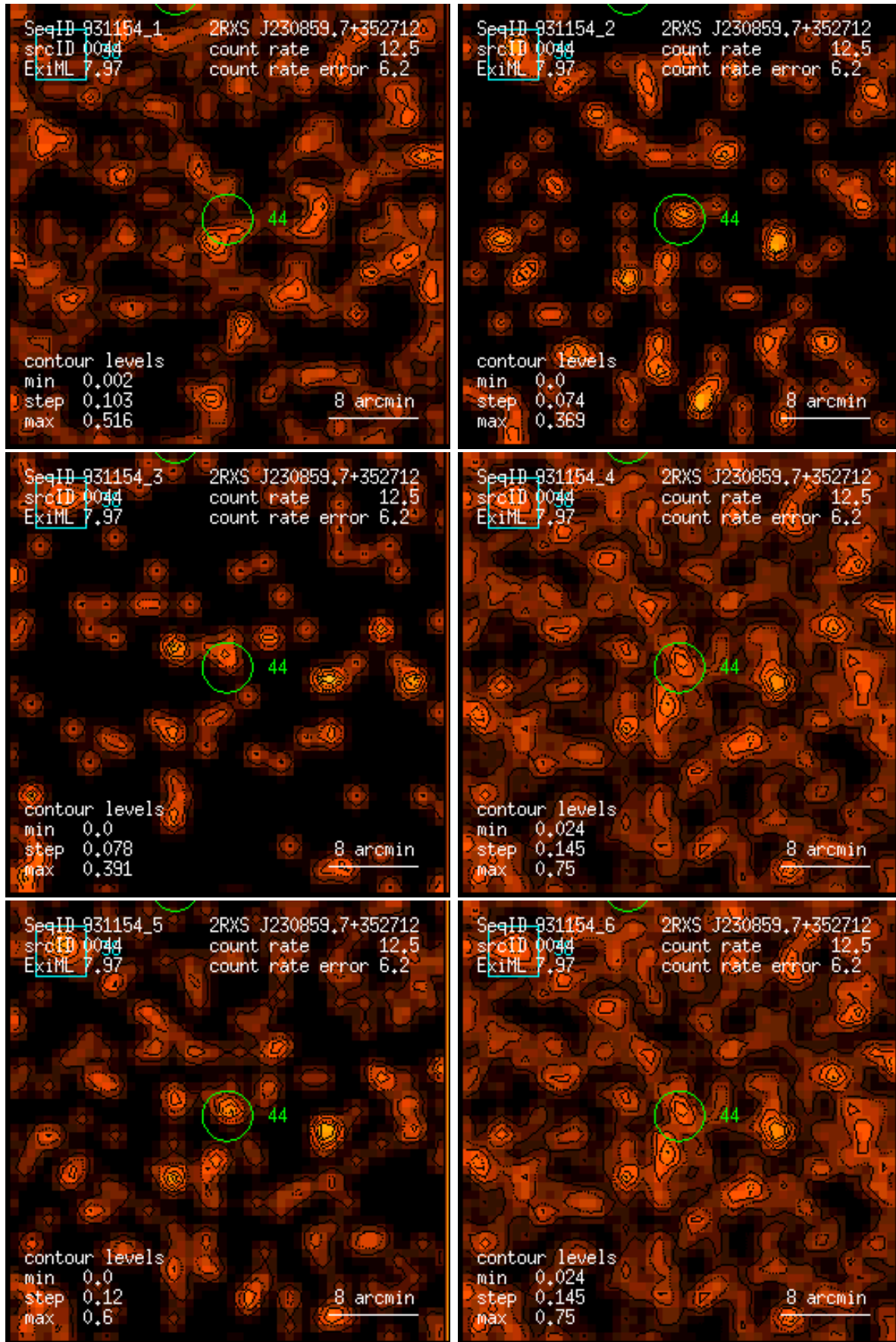
Figure 44: RASS 931154: detection 0044: band rate images, Gaussian filter: (1) PSPC channels 11 – 41, (2) 52 – 90, (3) 91 – 201, (4) 11 – 235, (5) 52 – 201, (6) 11 – 201. Broad band rates in counts/ks. Band rate contour levels in counts/ks/arcmin 2 .
