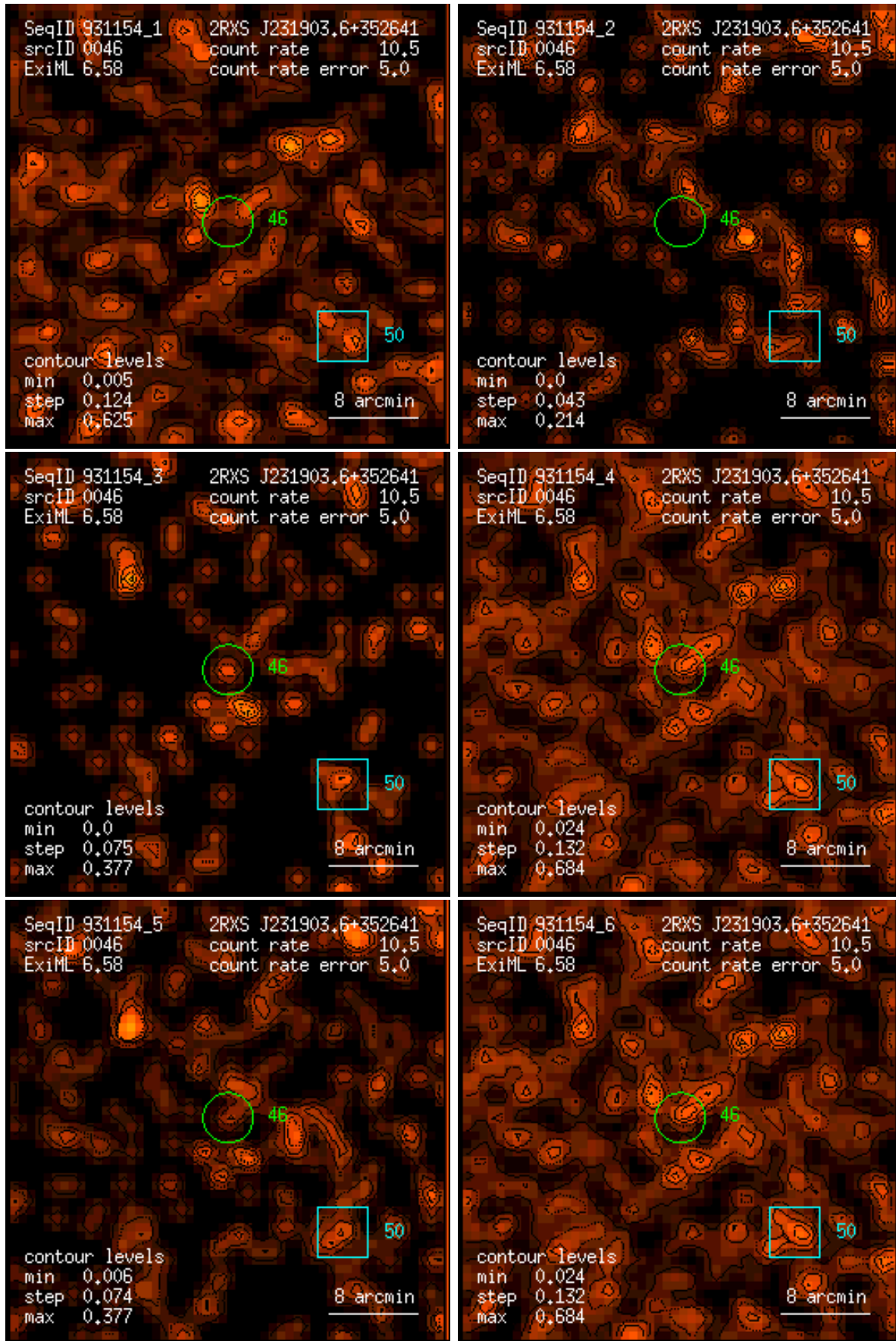
Figure 46: RASS 931154: detection 0046: band rate images, Gaussian filter: (1) PSPC channels 11 – 41, (2) 52 – 90, (3) 91 – 201, (4) 11 – 235, (5) 52 – 201, (6) 11 – 201. Broad band rates in counts/ks. Band rate contour levels in counts/ks/arcmin 2 .
