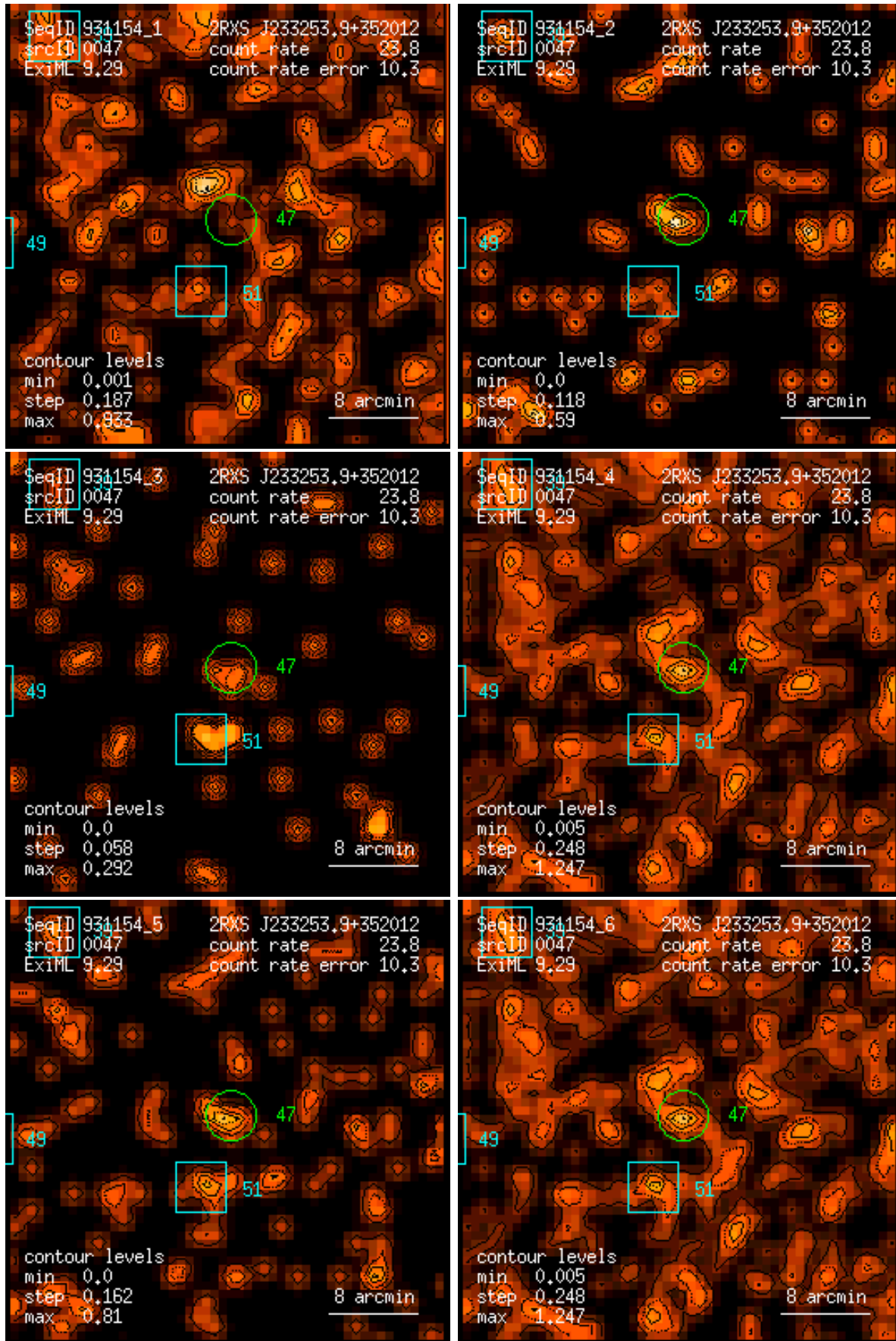
Figure 47: RASS 931154: detection 0047: band rate images, Gaussian filter: (1) PSPC channels 11 – 41, (2) 52 – 90, (3) 91 – 201, (4) 11 – 235, (5) 52 – 201, (6) 11 – 201. Broad band rates in counts/ks. Band rate contour levels in counts/ks/arcmin 2 .
