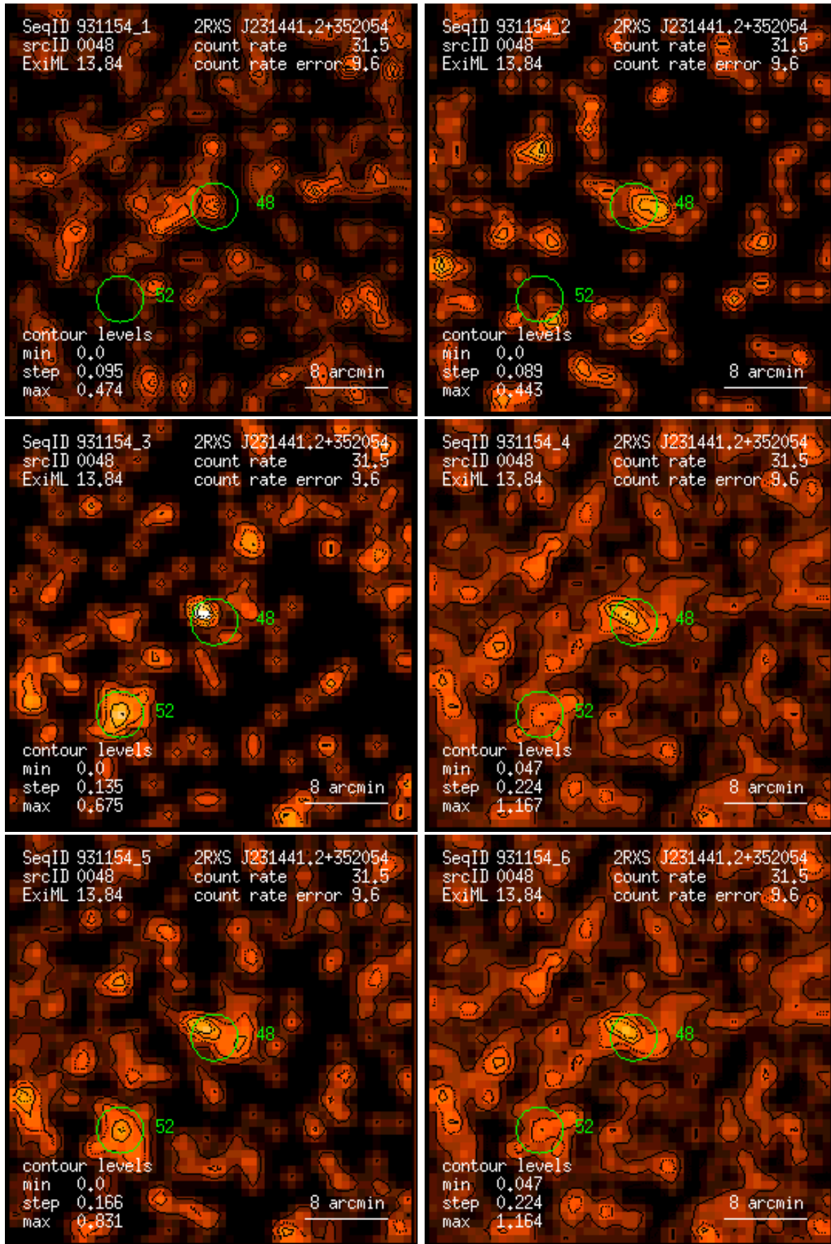
Figure 48: RASS 931154: detection 0048: band rate images, Gaussian filter: (1) PSPC channels 11 – 41, (2) 52 – 90, (3) 91 – 201, (4) 11 – 235, (5) 52 – 201, (6) 11 – 201. Broad band rates in counts/ks. Band rate contour levels in counts/ks/arcmin 2 .
