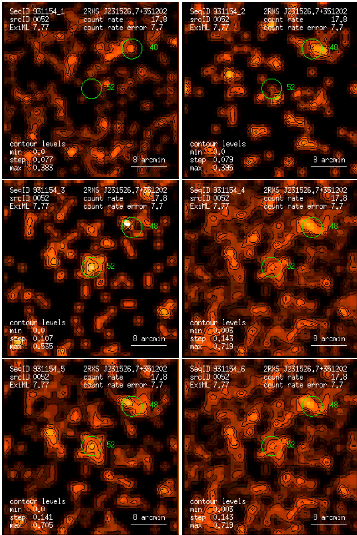
Figure 52: RASS 931154: detection 0052: band rate images, Gaussian filter: (1) PSPC channels 11 – 41, (2) 52 – 90, (3) 91 – 201, (4) 11 – 235, (5) 52 – 201, (6) 11 – 201. Broad band rates in counts/ks. Band rate contour levels in counts/ks/arcmin 2 .
