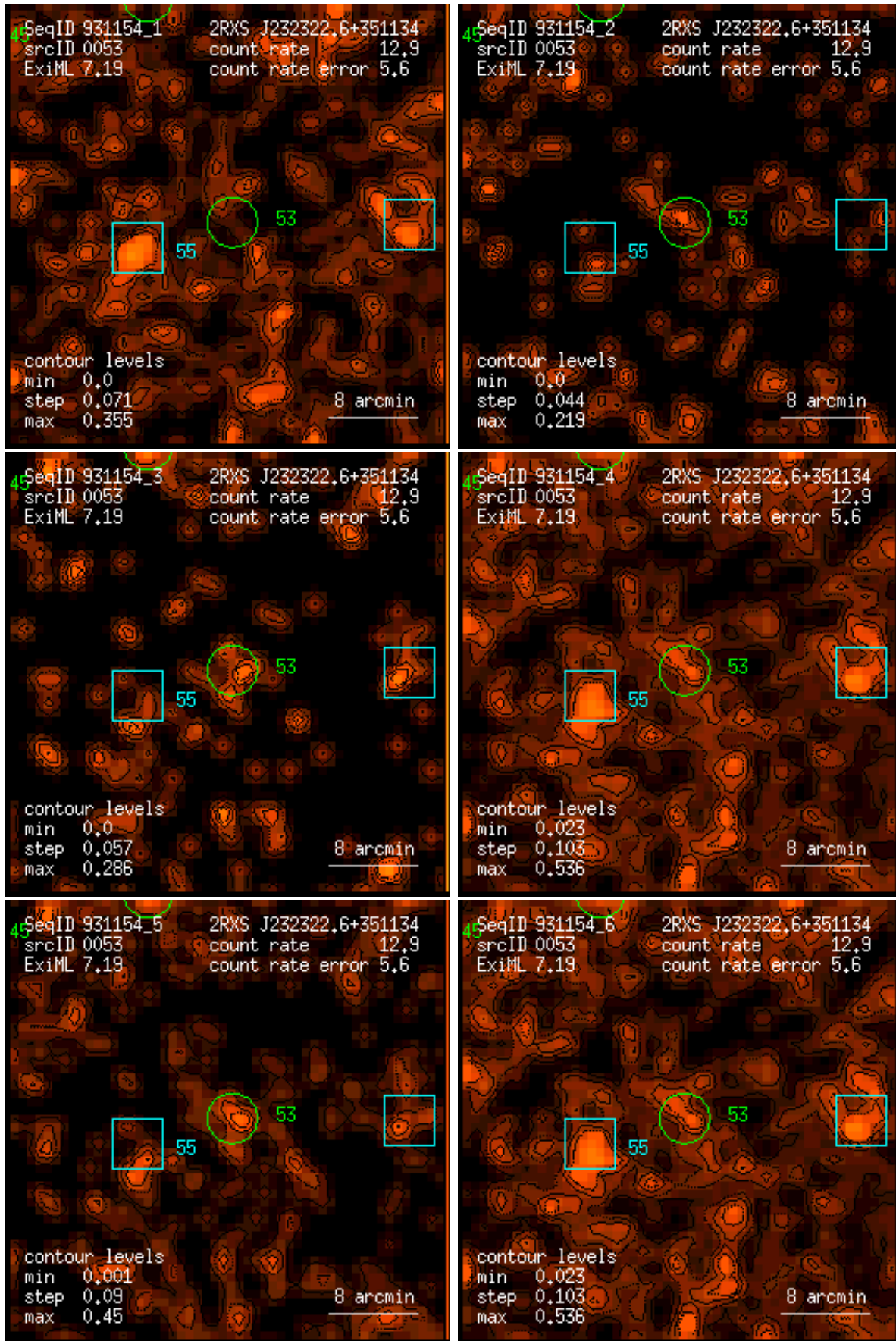
Figure 53: RASS 931154: detection 0053: band rate images, Gaussian filter: (1) PSPC channels 11 – 41, (2) 52 – 90, (3) 91 – 201, (4) 11 – 235, (5) 52 – 201, (6) 11 – 201. Broad band rates in counts/ks. Band rate contour levels in counts/ks/arcmin 2 .
