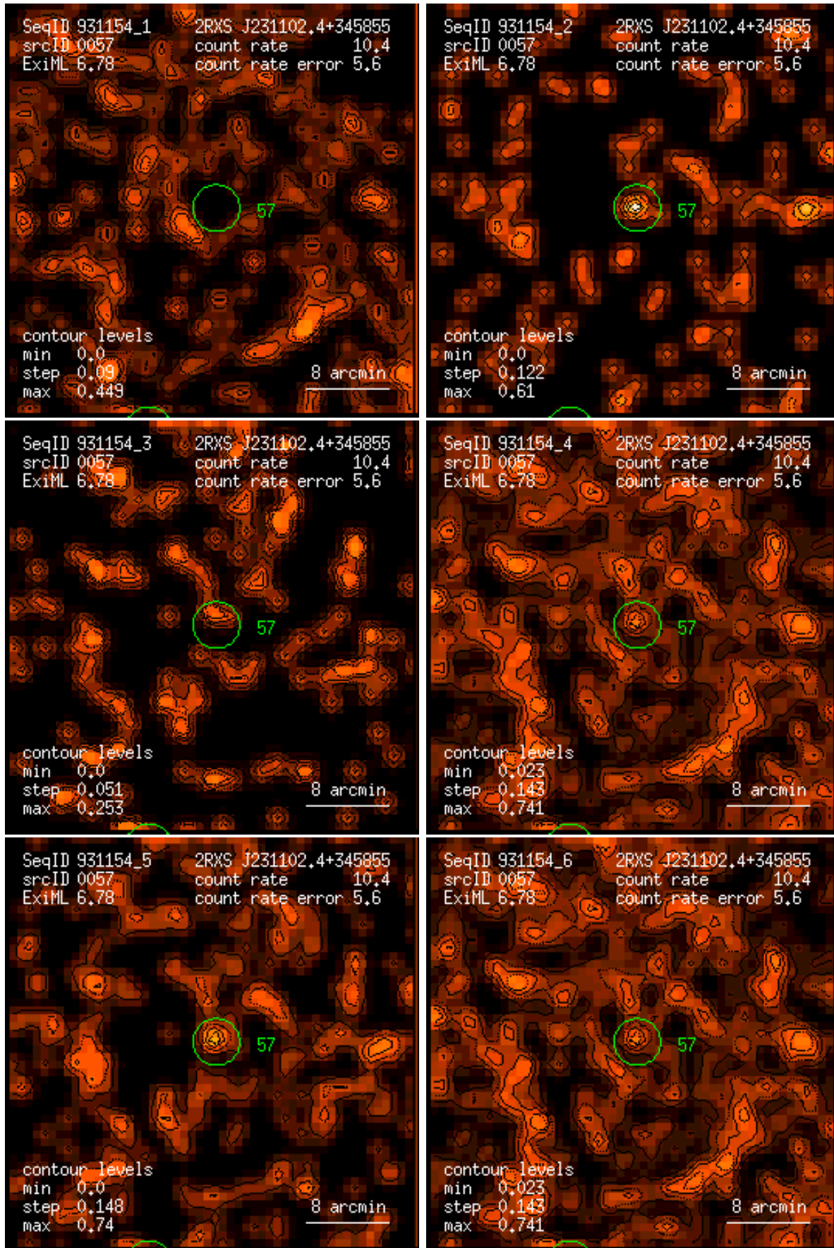
Figure 57: RASS 931154: detection 0057: band rate images, Gaussian filter: (1) PSPC channels 11 – 41, (2) 52 – 90, (3) 91 – 201, (4) 11 – 235, (5) 52 – 201, (6) 11 – 201. Broad band rates in counts/ks. Band rate contour levels in counts/ks/arcmin 2 .
