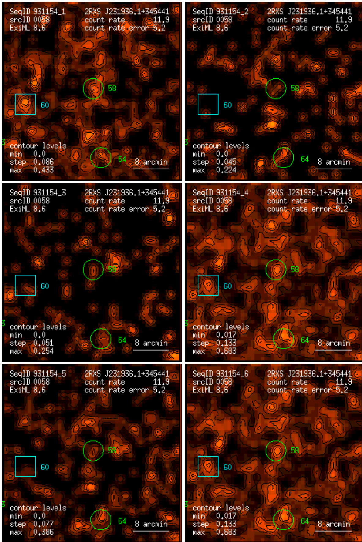
Figure 58: RASS 931154: detection 0058: band rate images, Gaussian filter: (1) PSPC channels 11 – 41, (2) 52 – 90, (3) 91 – 201, (4) 11 – 235, (5) 52 – 201, (6) 11 – 201. Broad band rates in counts/ks. Band rate contour levels in counts/ks/arcmin 2 .
