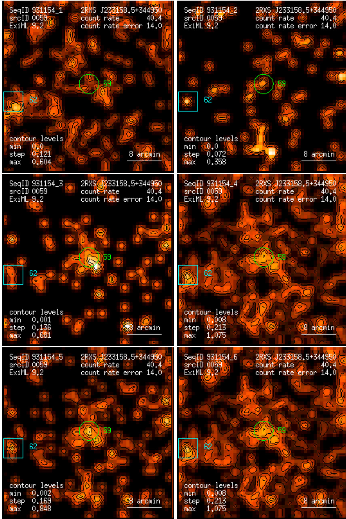
Figure 59: RASS 931154: detection 0059: band rate images, Gaussian filter: (1) PSPC channels 11 – 41, (2) 52 – 90, (3) 91 – 201, (4) 11 – 235, (5) 52 – 201, (6) 11 – 201. Broad band rates in counts/ks. Band rate contour levels in counts/ks/arcmin 2 .
