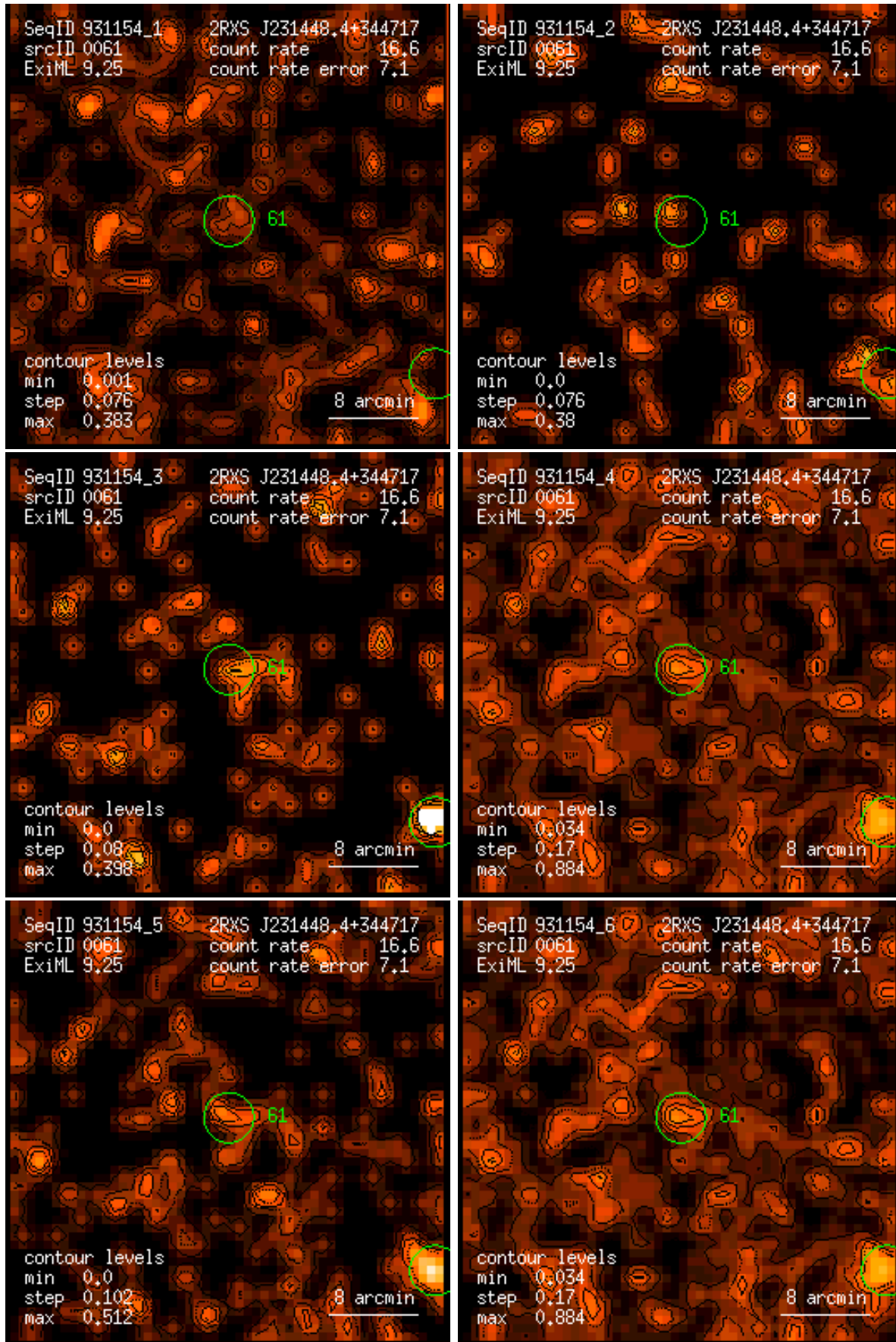
Figure 61: RASS 931154: detection 0061: band rate images, Gaussian filter: (1) PSPC channels 11 – 41, (2) 52 – 90, (3) 91 – 201, (4) 11 – 235, (5) 52 – 201, (6) 11 – 201. Broad band rates in counts/ks. Band rate contour levels in counts/ks/arcmin 2 .
