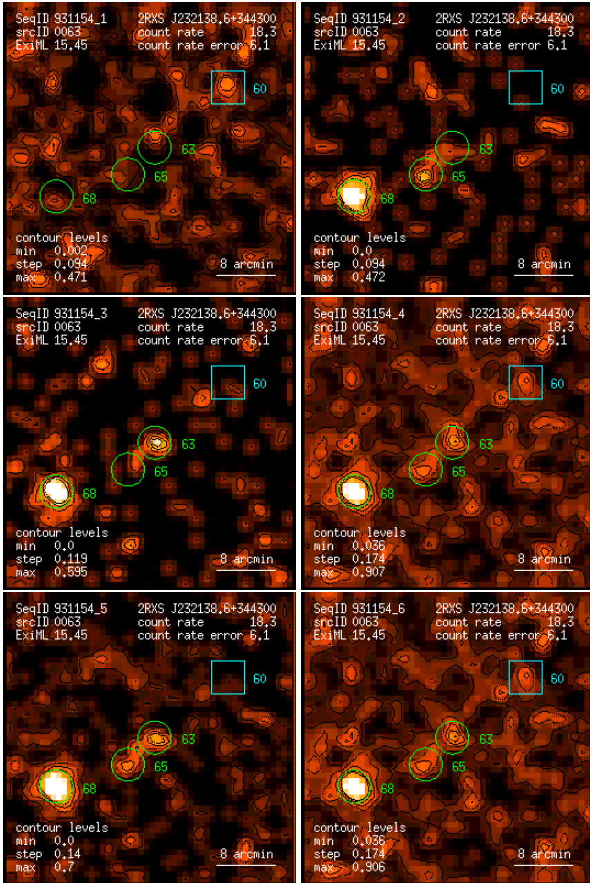
Figure 63: RASS 931154: detection 0063: band rate images, Gaussian filter: (1) PSPC channels 11 – 41, (2) 52 – 90, (3) 91 – 201, (4) 11 – 235, (5) 52 – 201, (6) 11 – 201. Broad band rates in counts/ks. Band rate contour levels in counts/ks/arcmin 2 .
