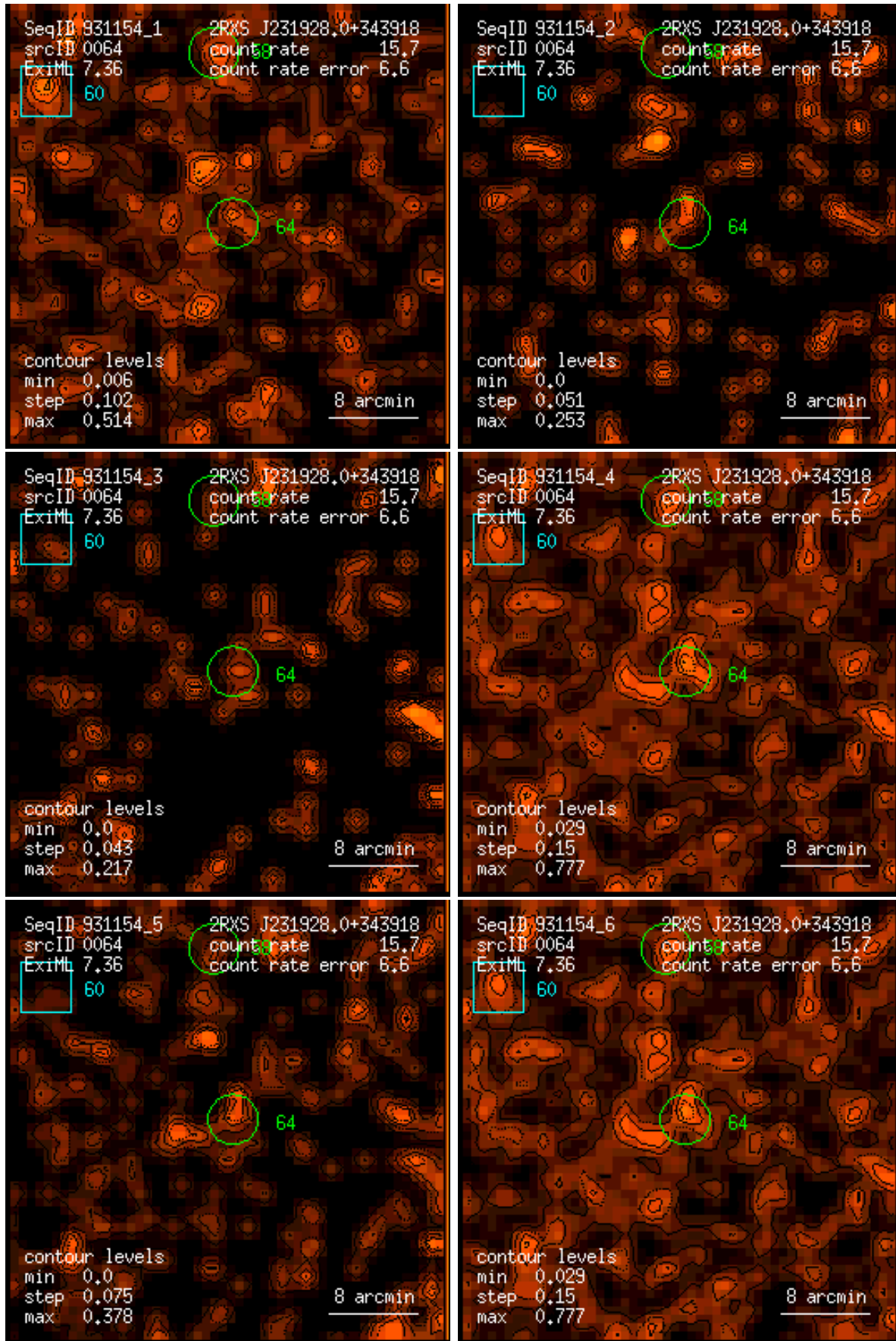
Figure 64: RASS 931154: detection 0064: band rate images, Gaussian filter: (1) PSPC channels 11 – 41, (2) 52 – 90, (3) 91 – 201, (4) 11 – 235, (5) 52 – 201, (6) 11 – 201. Broad band rates in counts/ks. Band rate contour levels in counts/ks/arcmin 2 .
