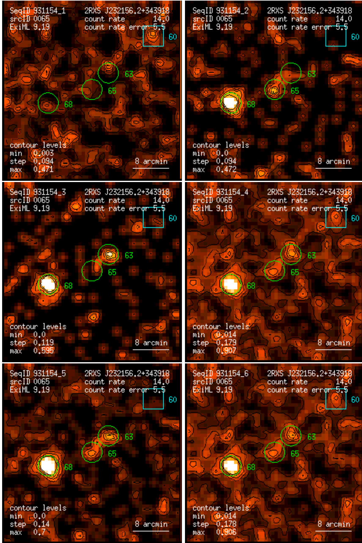
Figure 65: RASS 931154: detection 0065: band rate images, Gaussian filter: (1) PSPC channels 11 – 41, (2) 52 – 90, (3) 91 – 201, (4) 11 – 235, (5) 52 – 201, (6) 11 – 201. Broad band rates in counts/ks. Band rate contour levels in counts/ks/arcmin 2 .
