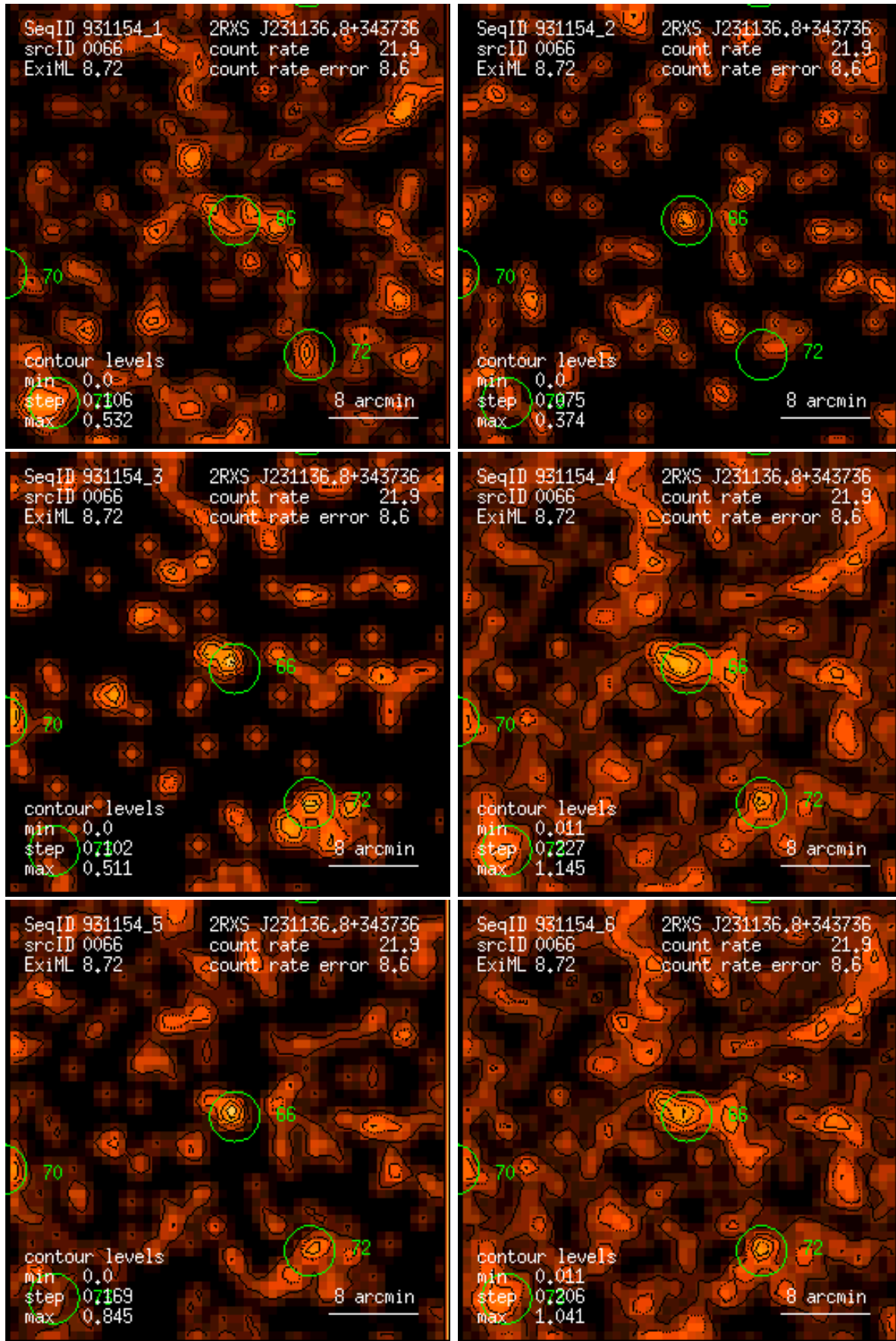
Figure 66: RASS 931154: detection 0066: band rate images, Gaussian filter: (1) PSPC channels 11 – 41, (2) 52 – 90, (3) 91 – 201, (4) 11 – 235, (5) 52 – 201, (6) 11 – 201. Broad band rates in counts/ks. Band rate contour levels in counts/ks/arcmin 2 .
