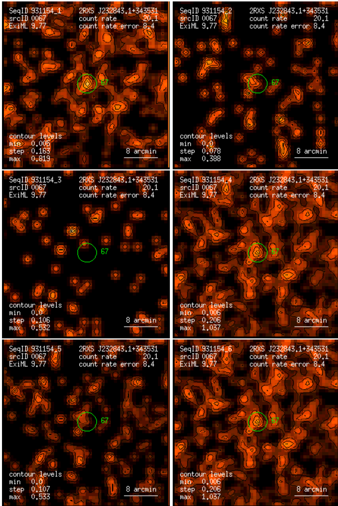
Figure 67: RASS 931154: detection 0067: band rate images, Gaussian filter: (1) PSPC channels 11 – 41, (2) 52 – 90, (3) 91 – 201, (4) 11 – 235, (5) 52 – 201, (6) 11 – 201. Broad band rates in counts/ks. Band rate contour levels in counts/ks/arcmin 2 .
