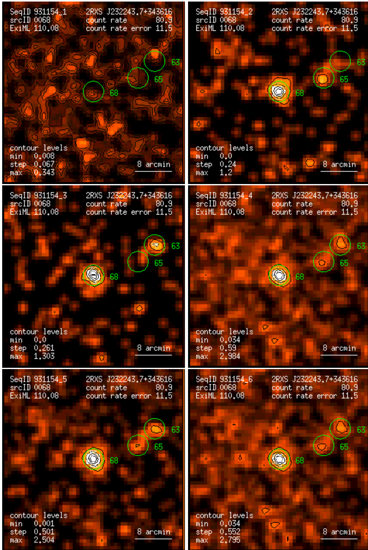
Figure 68: RASS 931154: detection 0068: band rate images, Gaussian filter: (1) PSPC channels 11 – 41, (2) 52 – 90, (3) 91 – 201, (4) 11 – 235, (5) 52 – 201, (6) 11 – 201. Broad band rates in counts/ks. Band rate contour levels in counts/ks/arcmin 2 .
