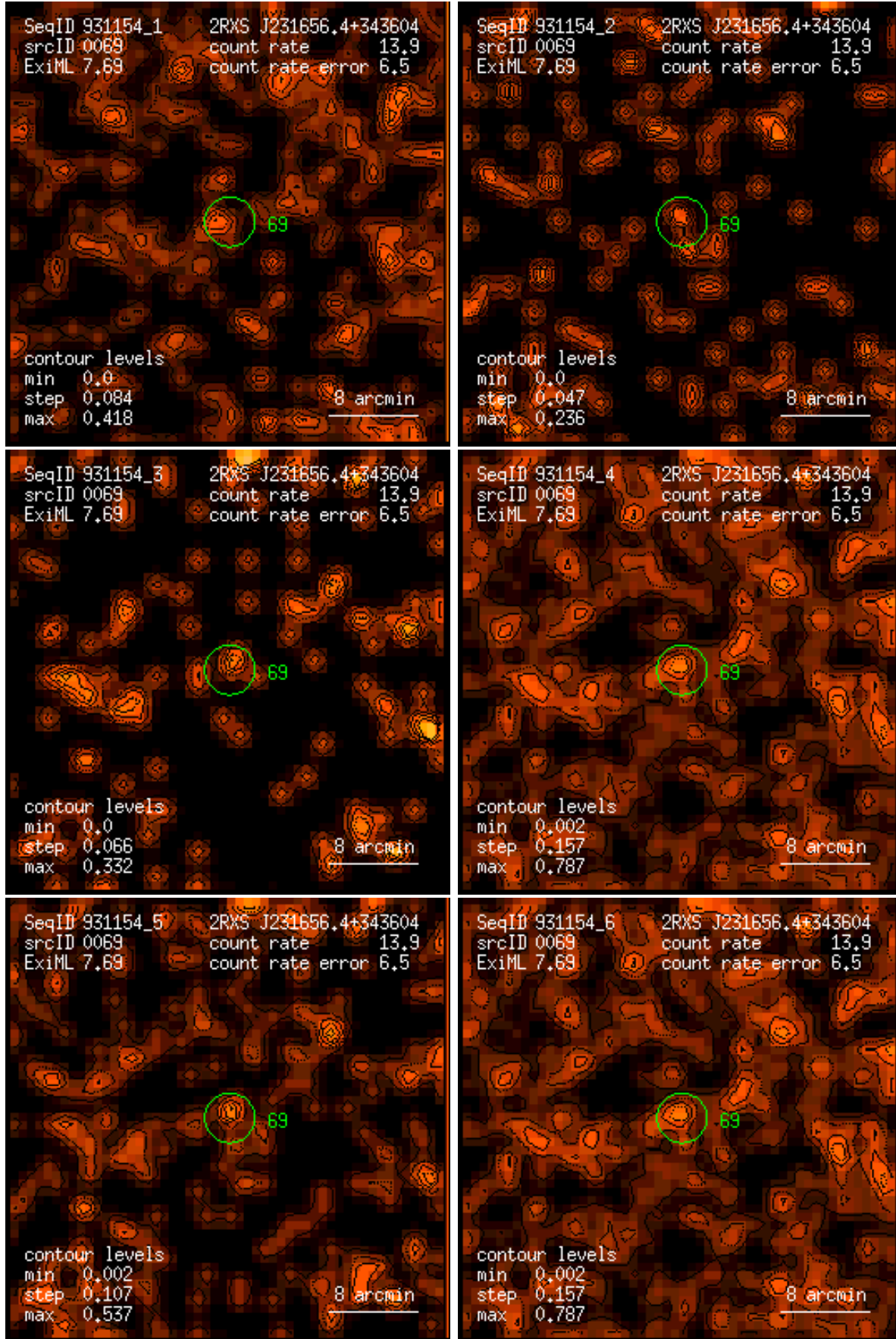
Figure 69: RASS 931154: detection 0069: band rate images, Gaussian filter: (1) PSPC channels 11 – 41, (2) 52 – 90, (3) 91 – 201, (4) 11 – 235, (5) 52 – 201, (6) 11 – 201. Broad band rates in counts/ks. Band rate contour levels in counts/ks/arcmin 2 .
