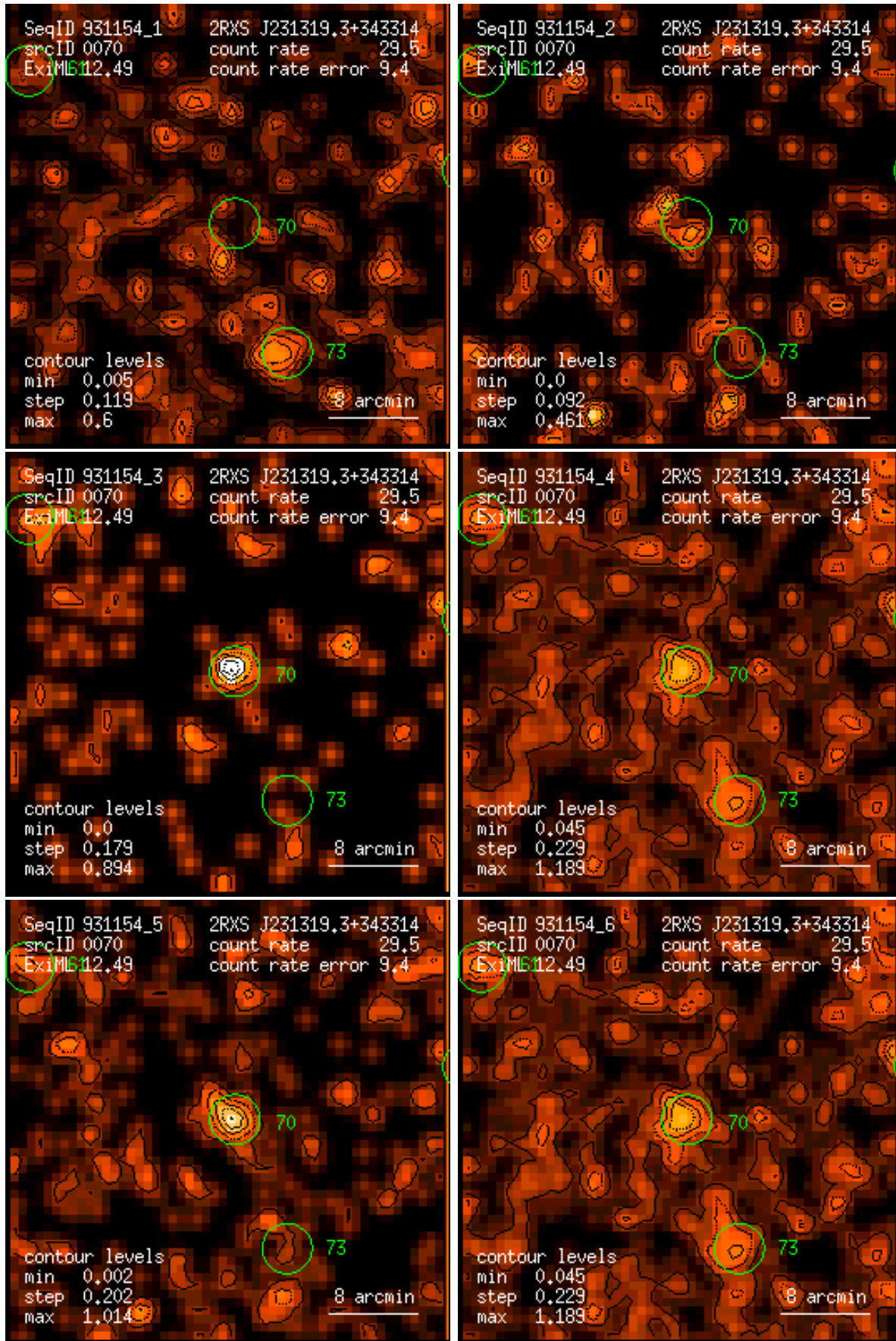
Figure 70: RASS 931154: detection 0070: band rate images, Gaussian filter: (1) PSPC channels 11 – 41, (2) 52 – 90, (3) 91 – 201, (4) 11 – 235, (5) 52 – 201, (6) 11 – 201. Broad band rates in counts/ks. Band rate contour levels in counts/ks/arcmin 2 .
