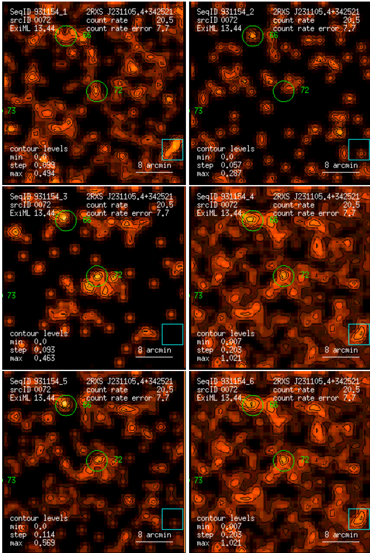
Figure 72: RASS 931154: detection 0072: band rate images, Gaussian filter: (1) PSPC channels 11 – 41, (2) 52 – 90, (3) 91 – 201, (4) 11 – 235, (5) 52 – 201, (6) 11 – 201. Broad band rates in counts/ks. Band rate contour levels in counts/ks/arcmin 2 .
