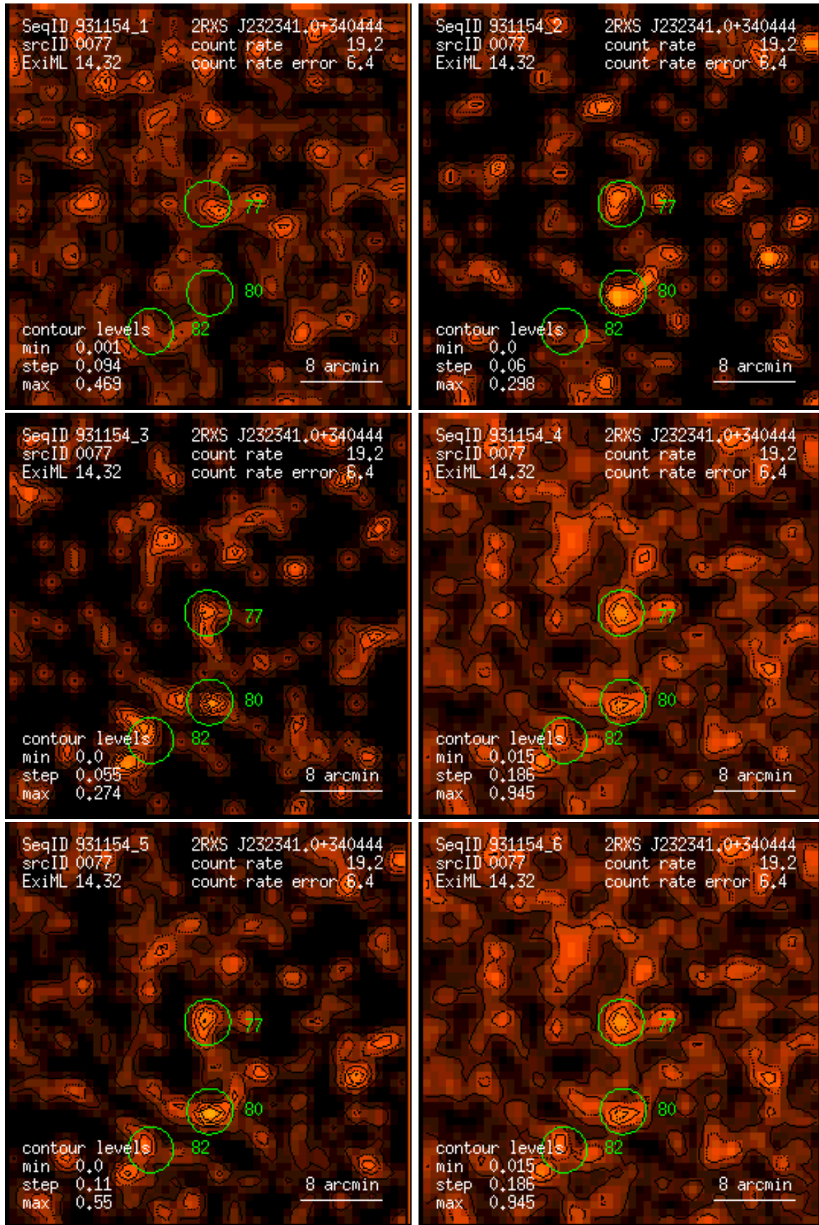
Figure 77: RASS 931154: detection 0077: band rate images, Gaussian filter: (1) PSPC channels 11 – 41, (2) 52 – 90, (3) 91 – 201, (4) 11 – 235, (5) 52 – 201, (6) 11 – 201. Broad band rates in counts/ks. Band rate contour levels in counts/ks/arcmin 2 .
