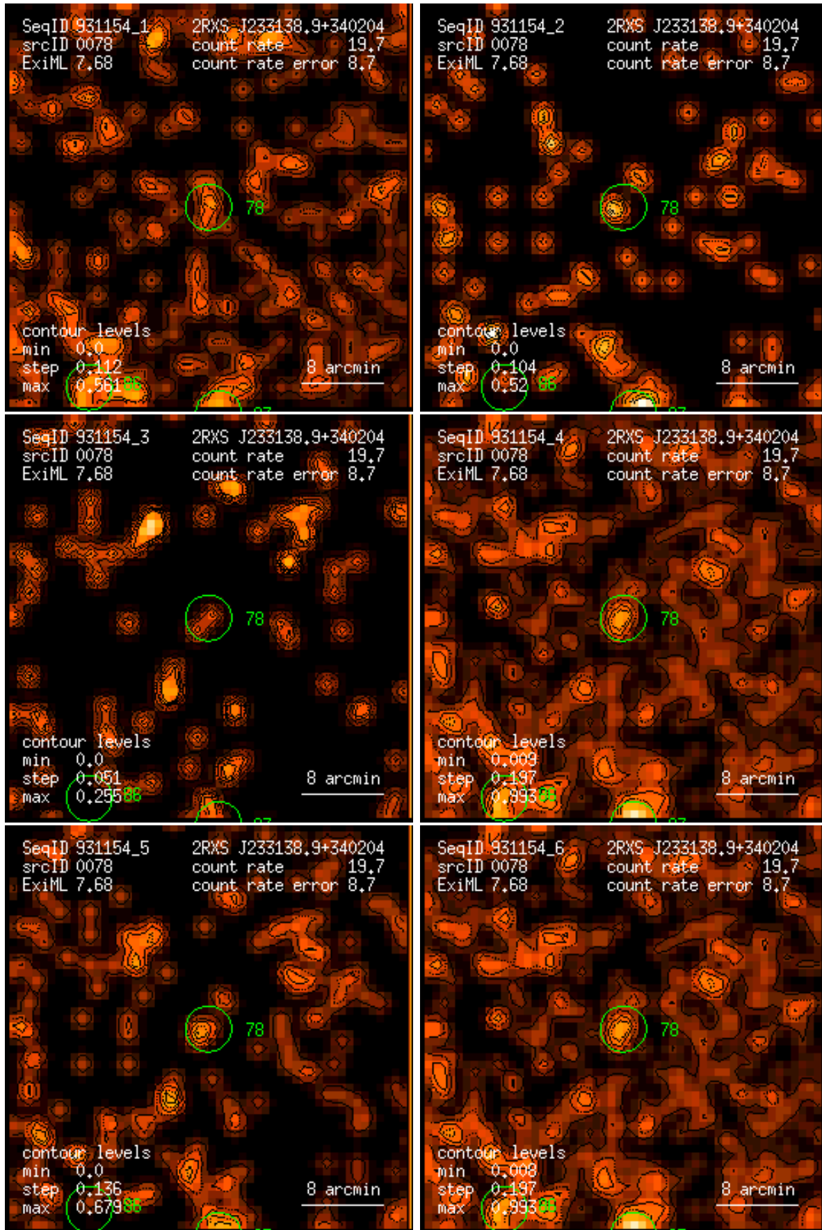
Figure 78: RASS 931154: detection 0078: band rate images, Gaussian filter: (1) PSPC channels 11 – 41, (2) 52 – 90, (3) 91 – 201, (4) 11 – 235, (5) 52 – 201, (6) 11 – 201. Broad band rates in counts/ks. Band rate contour levels in counts/ks/arcmin 2 .
