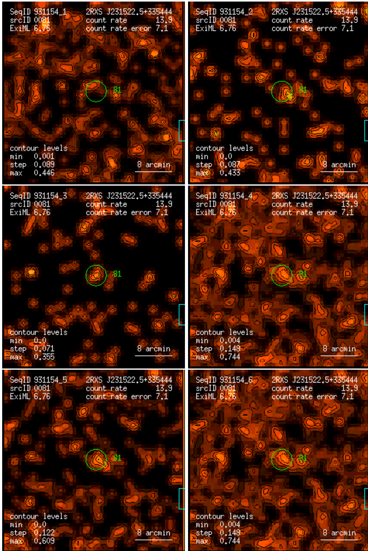
Figure 81: RASS 931154: detection 0081: band rate images, Gaussian filter: (1) PSPC channels 11 – 41, (2) 52 – 90, (3) 91 – 201, (4) 11 – 235, (5) 52 – 201, (6) 11 – 201. Broad band rates in counts/ks. Band rate contour levels in counts/ks/arcmin 2 .
