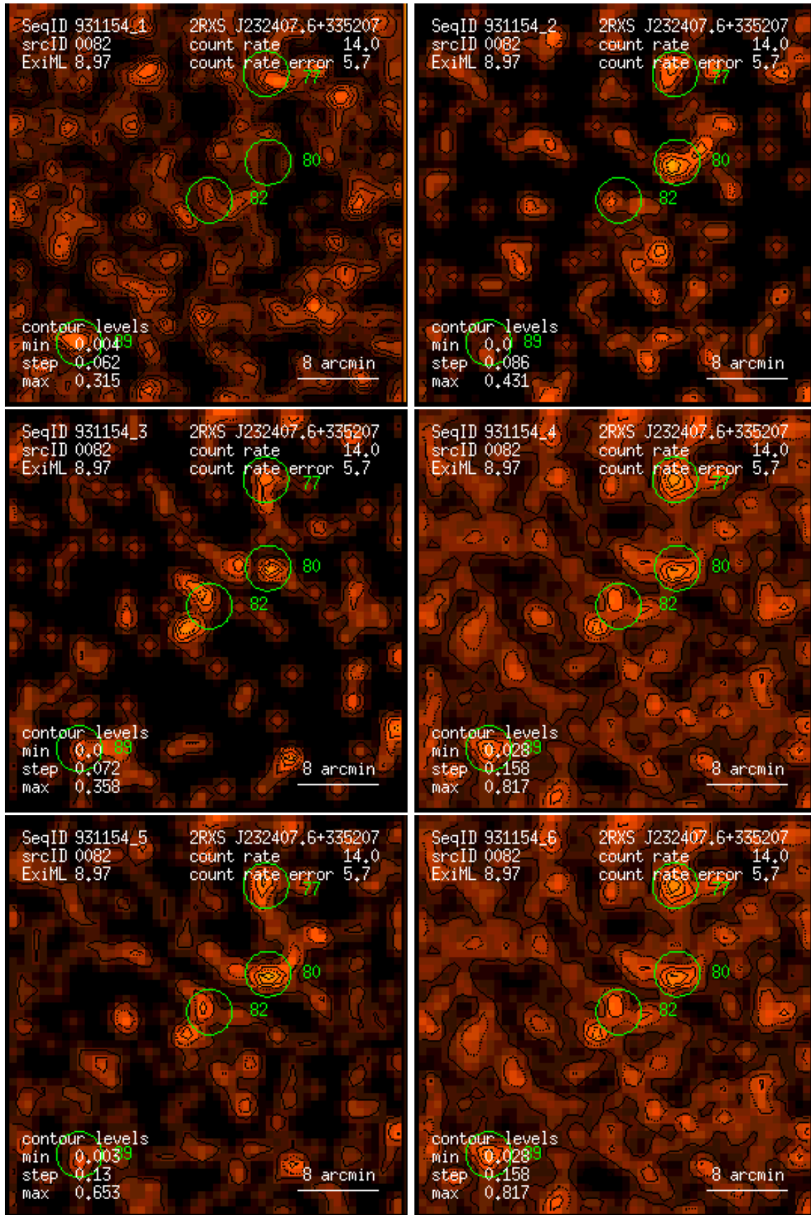
Figure 82: RASS 931154: detection 0082: band rate images, Gaussian filter: (1) PSPC channels 11 – 41, (2) 52 – 90, (3) 91 – 201, (4) 11 – 235, (5) 52 – 201, (6) 11 – 201. Broad band rates in counts/ks. Band rate contour levels in counts/ks/arcmin 2 .
