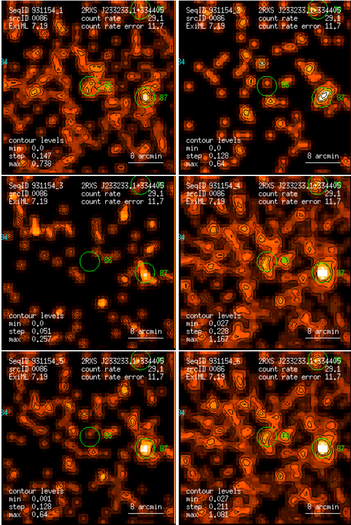
Figure 86: RASS 931154: detection 0086: band rate images, Gaussian filter: (1) PSPC channels 11 – 41, (2) 52 – 90, (3) 91 – 201, (4) 11 – 235, (5) 52 – 201, (6) 11 – 201. Broad band rates in counts/ks. Band rate contour levels in counts/ks/arcmin 2 .
