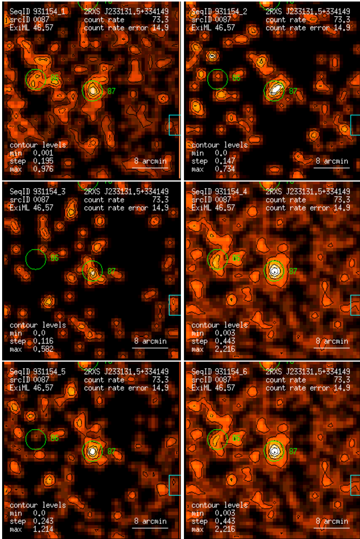
Figure 87: RASS 931154: detection 0087: band rate images, Gaussian filter: (1) PSPC channels 11 – 41, (2) 52 – 90, (3) 91 – 201, (4) 11 – 235, (5) 52 – 201, (6) 11 – 201. Broad band rates in counts/ks. Band rate contour levels in counts/ks/arcmin 2 .
