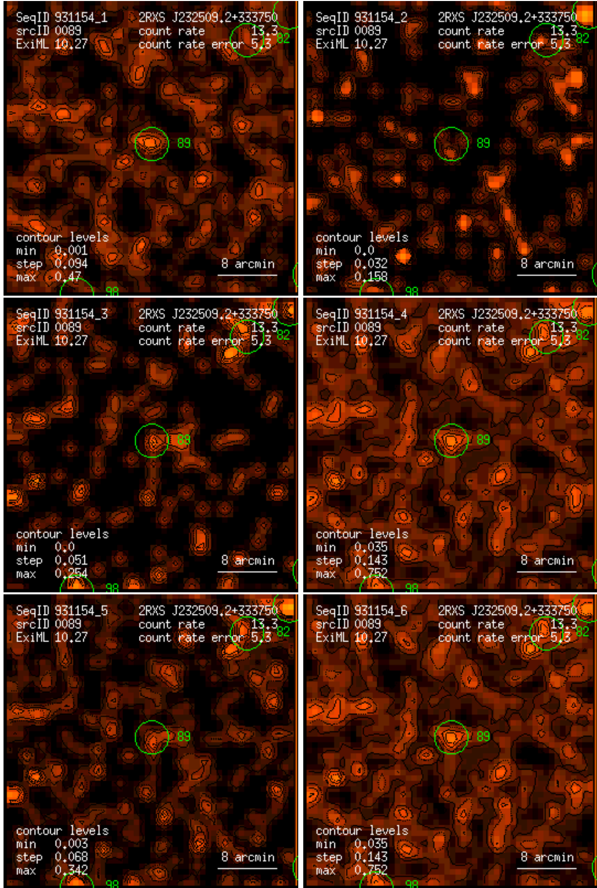
Figure 89: RASS 931154: detection 0089: band rate images, Gaussian filter: (1) PSPC channels 11 – 41, (2) 52 – 90, (3) 91 – 201, (4) 11 – 235, (5) 52 – 201, (6) 11 – 201. Broad band rates in counts/ks. Band rate contour levels in counts/ks/arcmin 2 .
