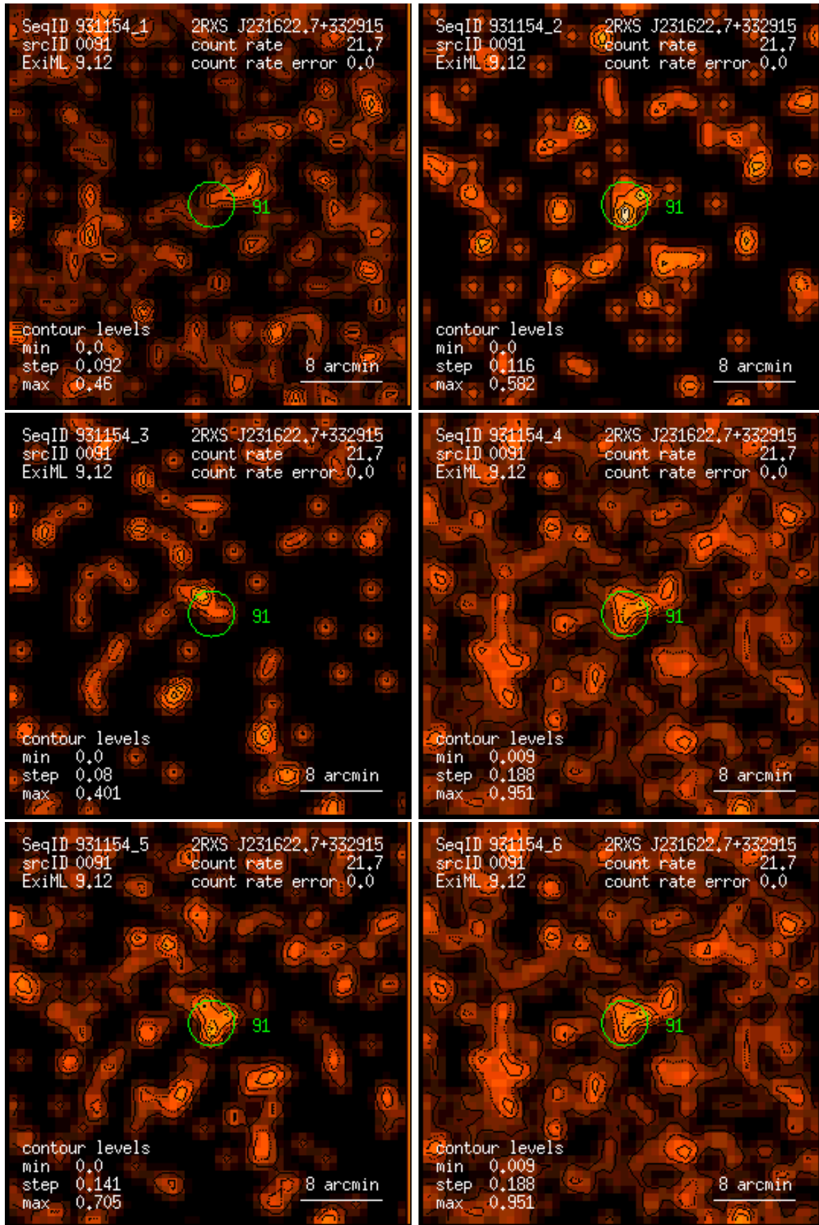
Figure 91: RASS 931154: detection 0091: band rate images, Gaussian filter: (1) PSPC channels 11 – 41, (2) 52 – 90, (3) 91 – 201, (4) 11 – 235, (5) 52 – 201, (6) 11 – 201. Broad band rates in counts/ks. Band rate contour levels in counts/ks/arcmin 2 .
