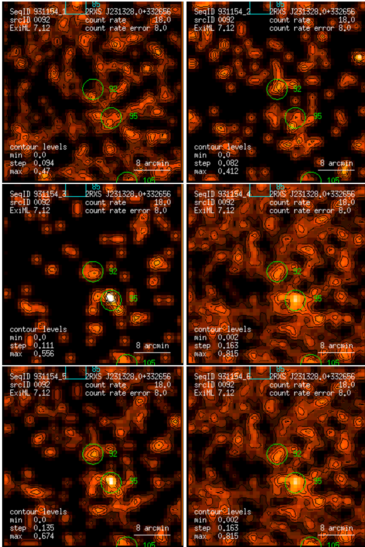
Figure 92: RASS 931154: detection 0092: band rate images, Gaussian filter: (1) PSPC channels 11 – 41, (2) 52 – 90, (3) 91 – 201, (4) 11 – 235, (5) 52 – 201, (6) 11 – 201. Broad band rates in counts/ks. Band rate contour levels in counts/ks/arcmin 2 .
