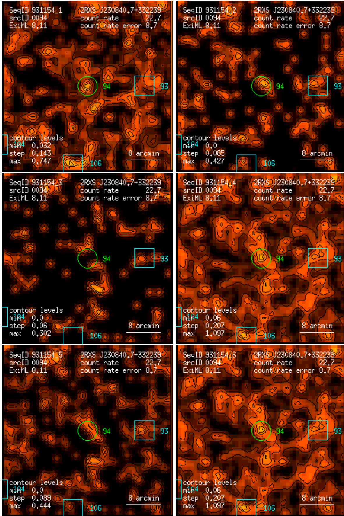
Figure 94: RASS 931154: detection 0094: band rate images, Gaussian filter: (1) PSPC channels 11 – 41, (2) 52 – 90, (3) 91 – 201, (4) 11 – 235, (5) 52 – 201, (6) 11 – 201. Broad band rates in counts/ks. Band rate contour levels in counts/ks/arcmin 2 .
