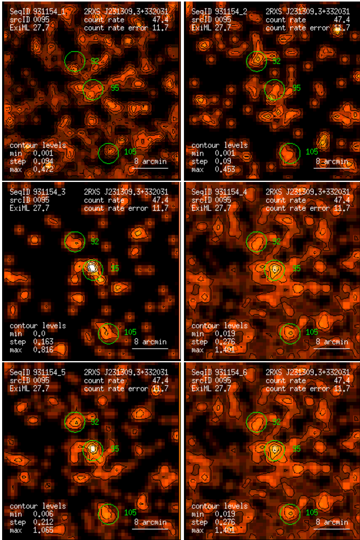
Figure 95: RASS 931154: detection 0095: band rate images, Gaussian filter: (1) PSPC channels 11 – 41, (2) 52 – 90, (3) 91 – 201, (4) 11 – 235, (5) 52 – 201, (6) 11 – 201. Broad band rates in counts/ks. Band rate contour levels in counts/ks/arcmin 2 .
