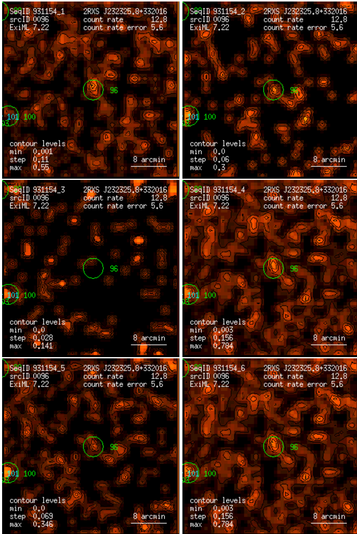
Figure 96: RASS 931154: detection 0096: band rate images, Gaussian filter: (1) PSPC channels 11 – 41, (2) 52 – 90, (3) 91 – 201, (4) 11 – 235, (5) 52 – 201, (6) 11 – 201. Broad band rates in counts/ks. Band rate contour levels in counts/ks/arcmin 2 .
