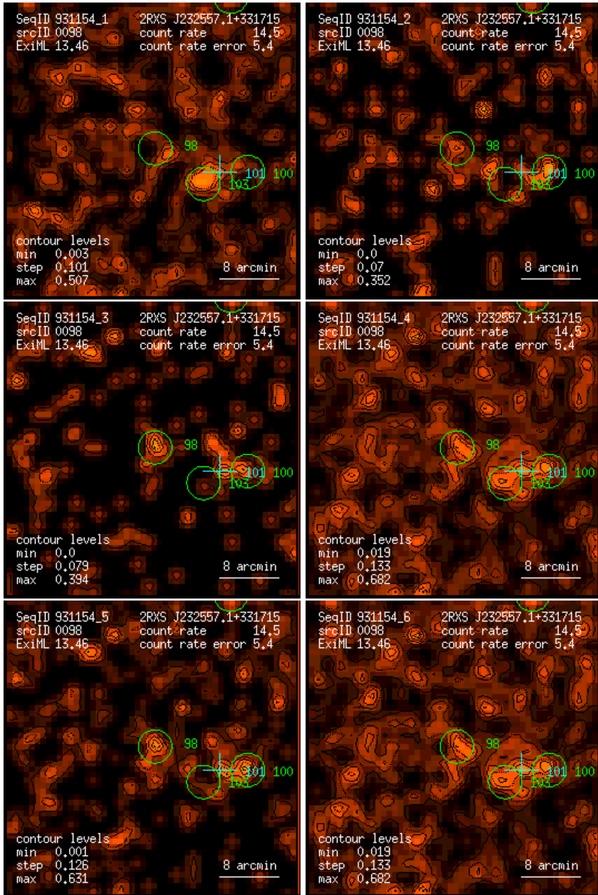
Figure 98: RASS 931154: detection 0098: band rate images, Gaussian filter: (1) PSPC channels 11 – 41, (2) 52 – 90, (3) 91 – 201, (4) 11 – 235, (5) 52 – 201, (6) 11 – 201. Broad band rates in counts/ks. Band rate contour levels in counts/ks/arcmin 2 .
