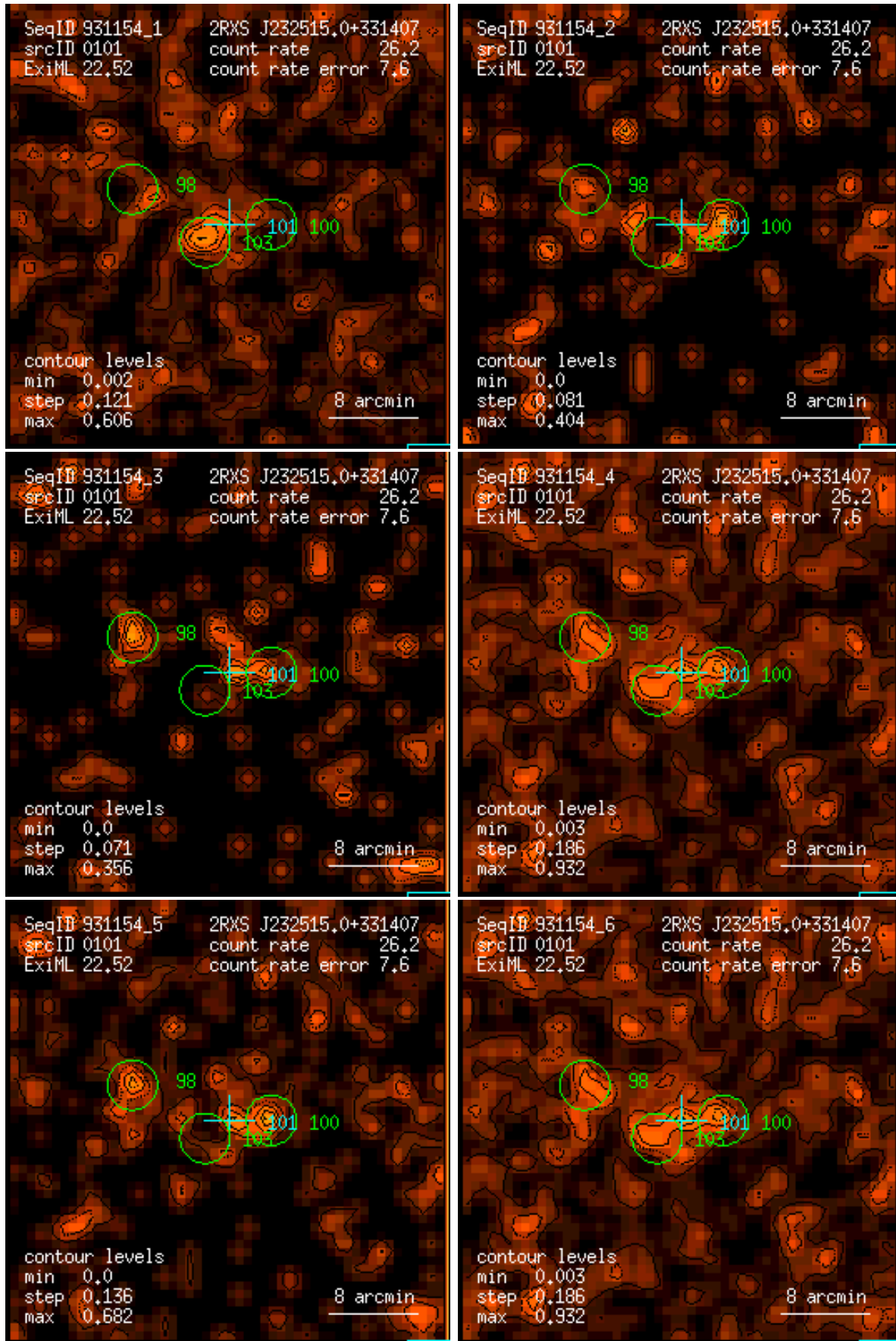
Figure 101: RASS 931154: detection 0101: band rate images, Gaussian filter: (1) PSPC channels 11 – 41, (2) 52 – 90, (3) 91 – 201, (4) 11 – 235, (5) 52 – 201, (6) 11 – 201. Broad band rates in counts/ks. Band rate contour levels in counts/ks/arcmin 2 .
