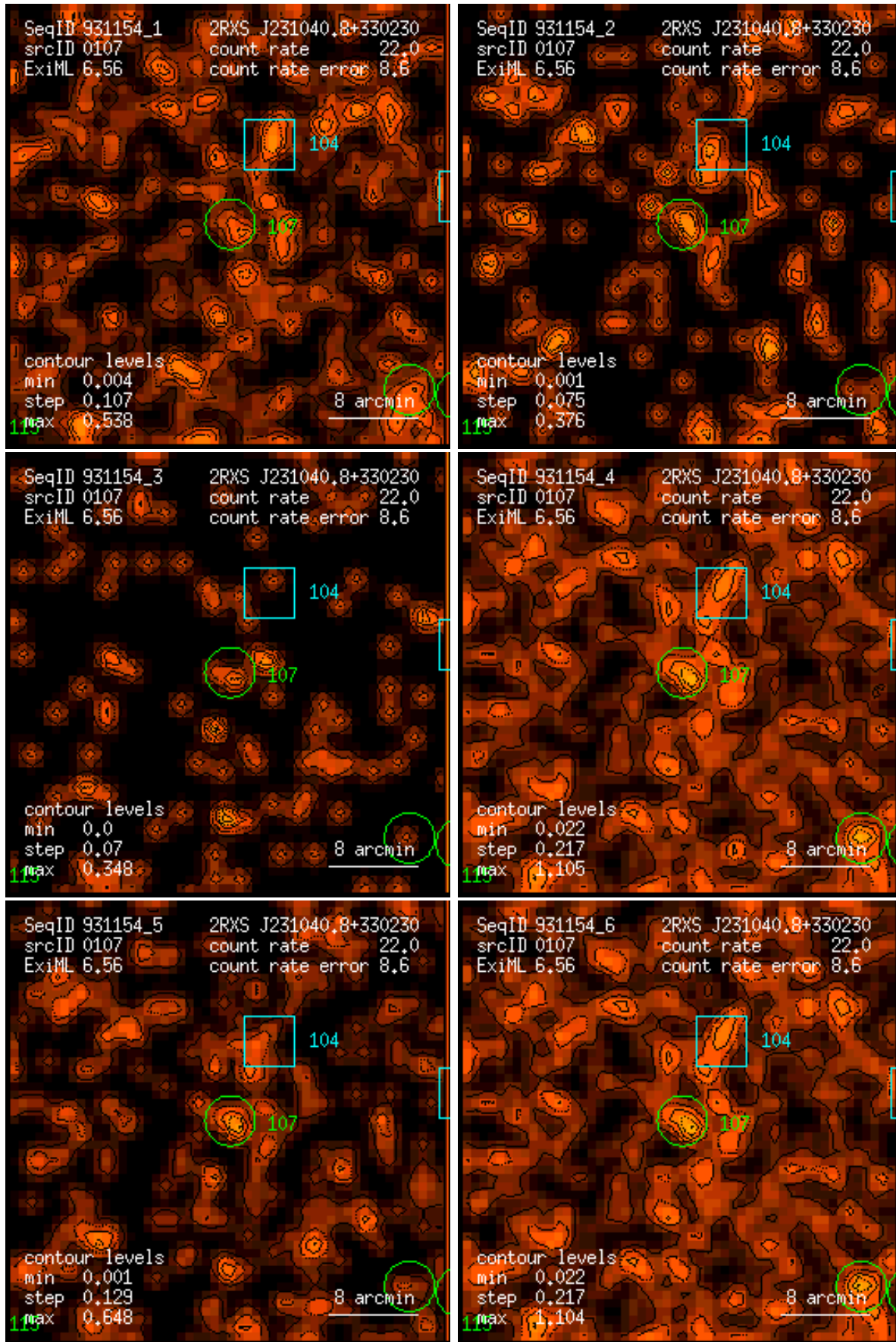
Figure 107: RASS 931154: detection 0107: band rate images, Gaussian filter: (1) PSPC channels 11 – 41, (2) 52 – 90, (3) 91 – 201, (4) 11 – 235, (5) 52 – 201, (6) 11 – 201. Broad band rates in counts/ks. Band rate contour levels in counts/ks/arcmin 2 .
