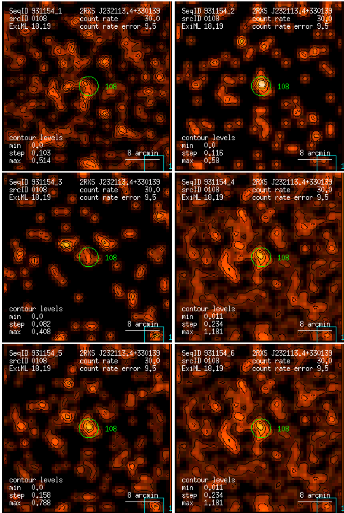
Figure 108: RASS 931154: detection 0108: band rate images, Gaussian filter: (1) PSPC channels 11 – 41, (2) 52 – 90, (3) 91 – 201, (4) 11 – 235, (5) 52 – 201, (6) 11 – 201. Broad band rates in counts/ks. Band rate contour levels in counts/ks/arcmin 2 .
