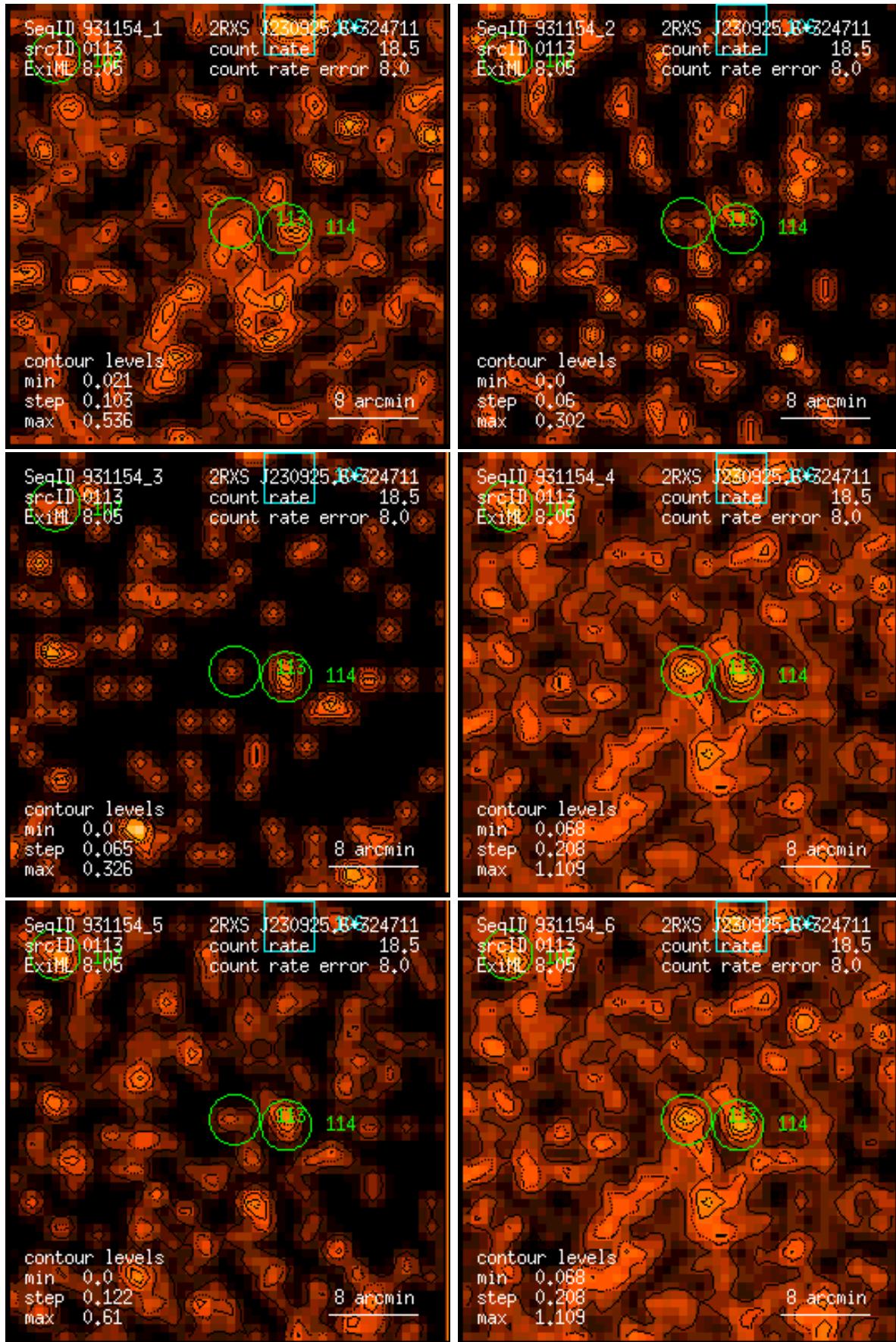
Figure 113: RASS 931154: detection 0113: band rate images, Gaussian filter: (1) PSPC channels 11 – 41, (2) 52 – 90, (3) 91 – 201, (4) 11 – 235, (5) 52 – 201, (6) 11 – 201. Broad band rates in counts/ks. Band rate contour levels in counts/ks/arcmin 2 .
