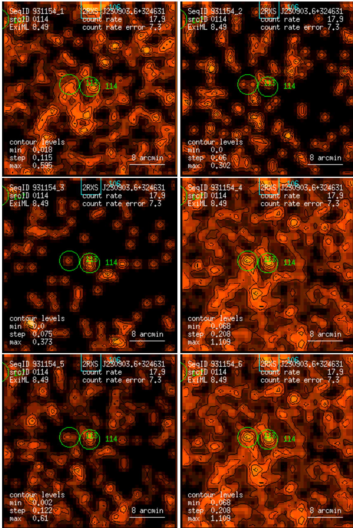
Figure 114: RASS 931154: detection 0114: band rate images, Gaussian filter: (1) PSPC channels 11 – 41, (2) 52 – 90, (3) 91 – 201, (4) 11 – 235, (5) 52 – 201, (6) 11 – 201. Broad band rates in counts/ks. Band rate contour levels in counts/ks/arcmin 2 .
