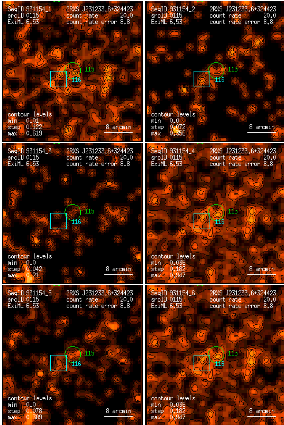
Figure 115: RASS 931154: detection 0115: band rate images, Gaussian filter: (1) PSPC channels 11 – 41, (2) 52 – 90, (3) 91 – 201, (4) 11 – 235, (5) 52 – 201, (6) 11 – 201. Broad band rates in counts/ks. Band rate contour levels in counts/ks/arcmin 2 .
