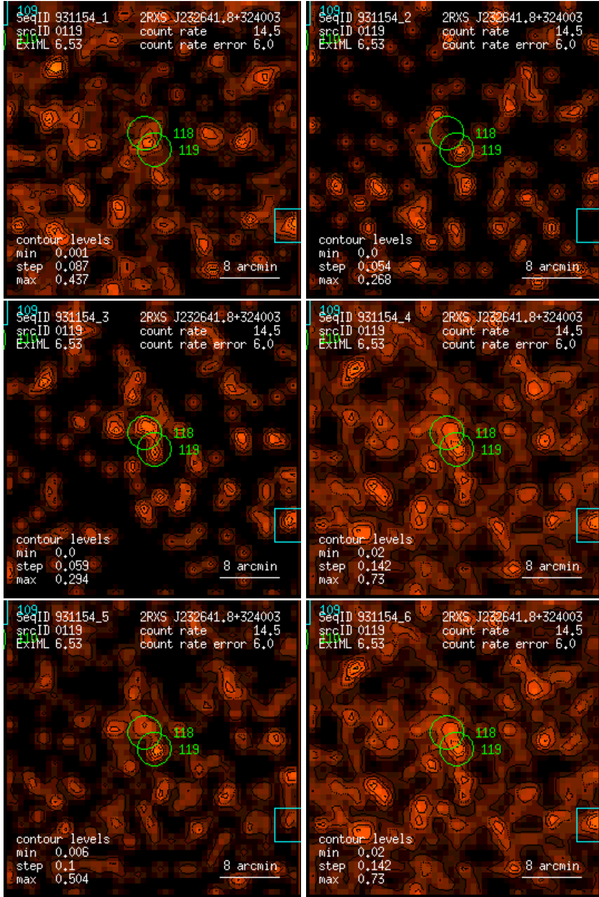
Figure 119: RASS 931154: detection 0119: band rate images, Gaussian filter: (1) PSPC channels 11 – 41, (2) 52 – 90, (3) 91 – 201, (4) 11 – 235, (5) 52 – 201, (6) 11 – 201. Broad band rates in counts/ks. Band rate contour levels in counts/ks/arcmin 2 .
