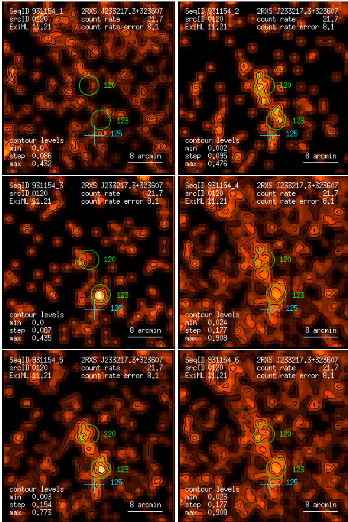
Figure 120: RASS 931154: detection 0120: band rate images, Gaussian filter: (1) PSPPC channels 11 – 41, (2) 52 – 90, (3) 91 – 201, (4) 11 – 235, (5) 52 – 201, (6) 11 – 201. Broad band rates in counts/ks. Band rate contour levels in counts/ks/arcmin 2 .
