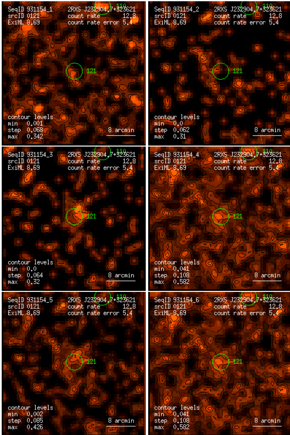
Figure 121: RASS 931154: detection 0121: band rate images, Gaussian filter: (1) PSPC channels 11 – 41, (2) 52 – 90, (3) 91 – 201, (4) 11 – 235, (5) 52 – 201, (6) 11 – 201. Broad band rates in counts/ks. Band rate contour levels in counts/ks/arcmin 2 .
