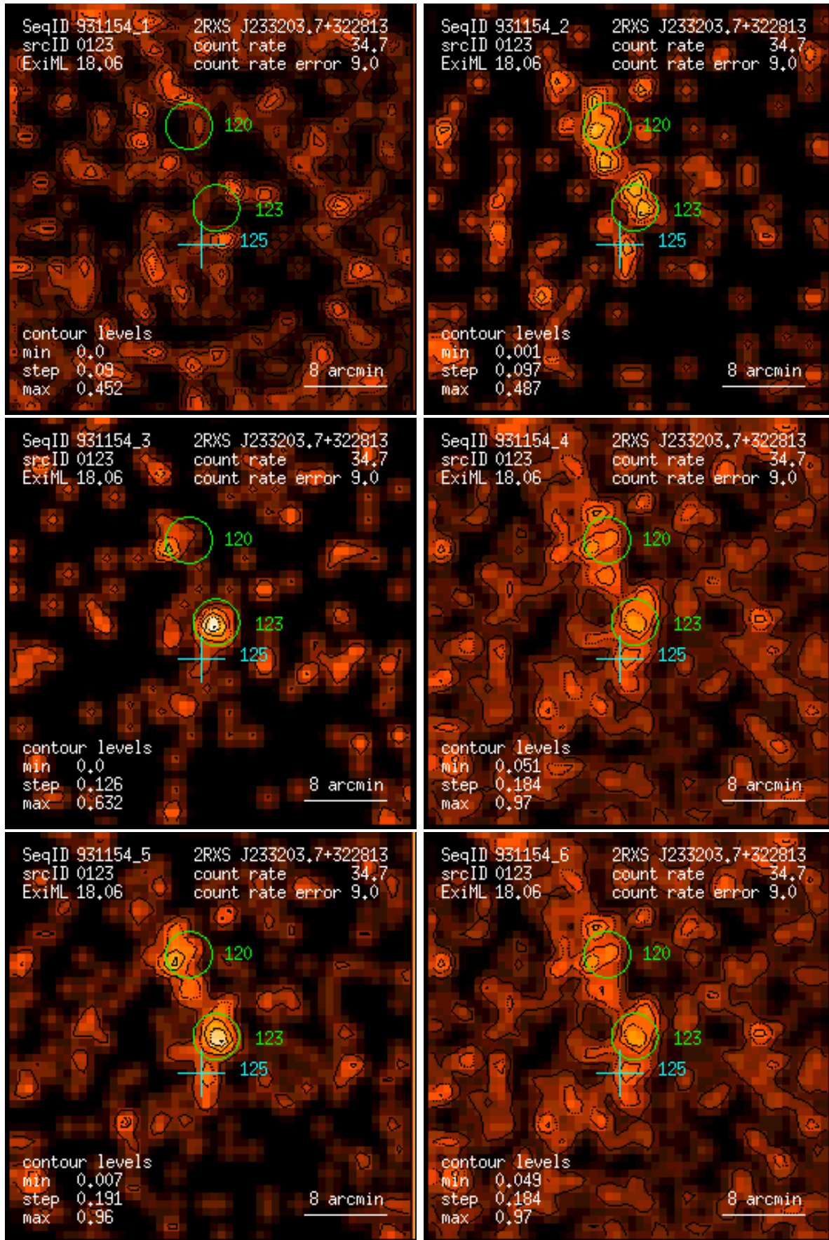
Figure 123: RASS 931154: detection 0123: band rate images, Gaussian filter: (1) PSPC channels 11 – 41, (2) 52 – 90, (3) 91 – 201, (4) 11 – 235, (5) 52 – 201, (6) 11 – 201. Broad band rates in counts/ks. Band rate contour levels in counts/ks/arcmin 2 .
