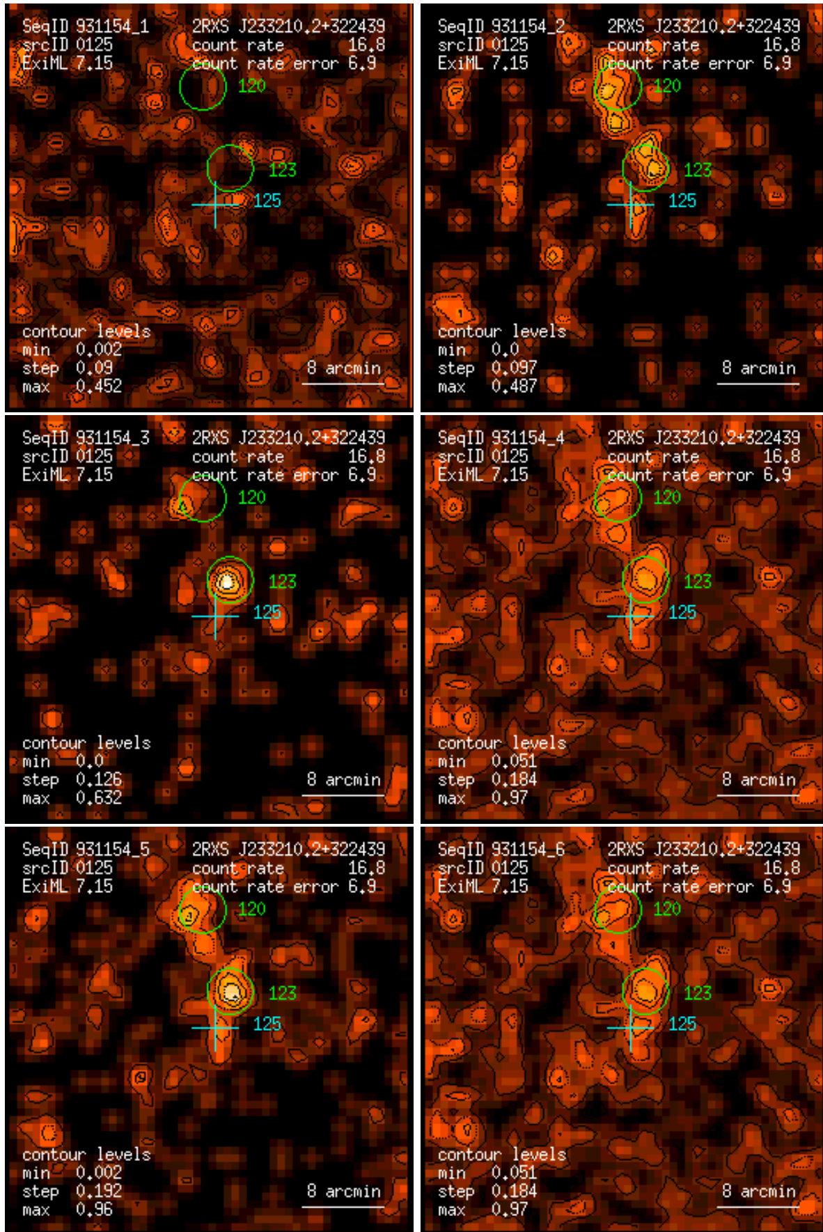
Figure 125: RASS 931154: detection 0125: band rate images, Gaussian filter: (1) PSPC channels 11 – 41, (2) 52 – 90, (3) 91 – 201, (4) 11 – 235, (5) 52 – 201, (6) 11 – 201. Broad band rates in counts/ks. Band rate contour levels in counts/ks/arcmin 2 .
