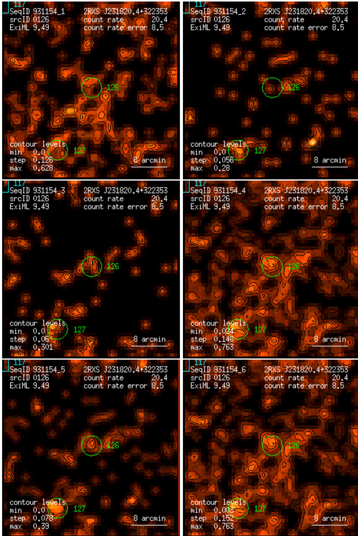
Figure 126: RASS 931154: detection 0126: band rate images, Gaussian filter: (1) PSPC channels 11 – 41, (2) 52 – 90, (3) 91 – 201, (4) 11 – 235, (5) 52 – 201, (6) 11 – 201. Broad band rates in counts/ks. Band rate contour levels in counts/ks/arcmin 2 .
