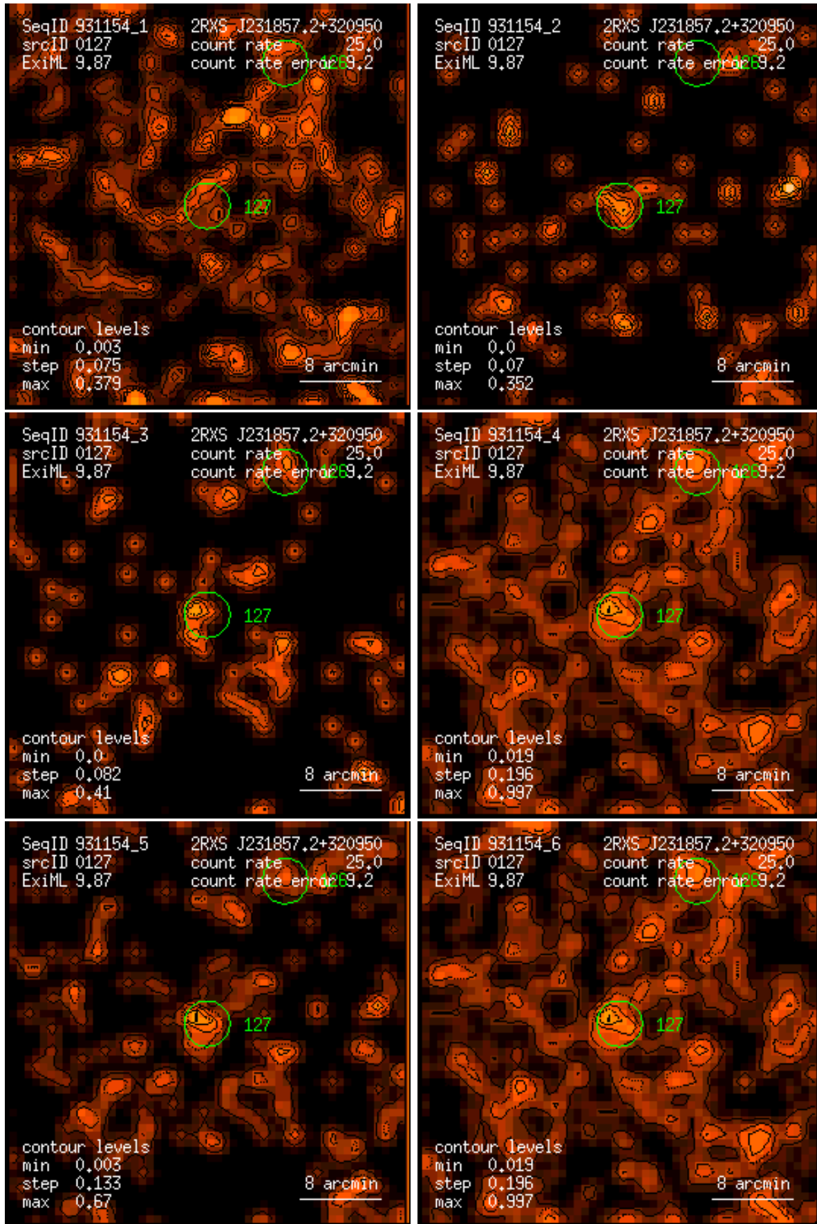
Figure 127: RASS 931154: detection 0127: band rate images, Gaussian filter: (1) PSPC channels 11 – 41, (2) 52 – 90, (3) 91 – 201, (4) 11 – 235, (5) 52 – 201, (6) 11 – 201. Broad band rates in counts/ks. Band rate contour levels in counts/ks/arcmin 2 .
