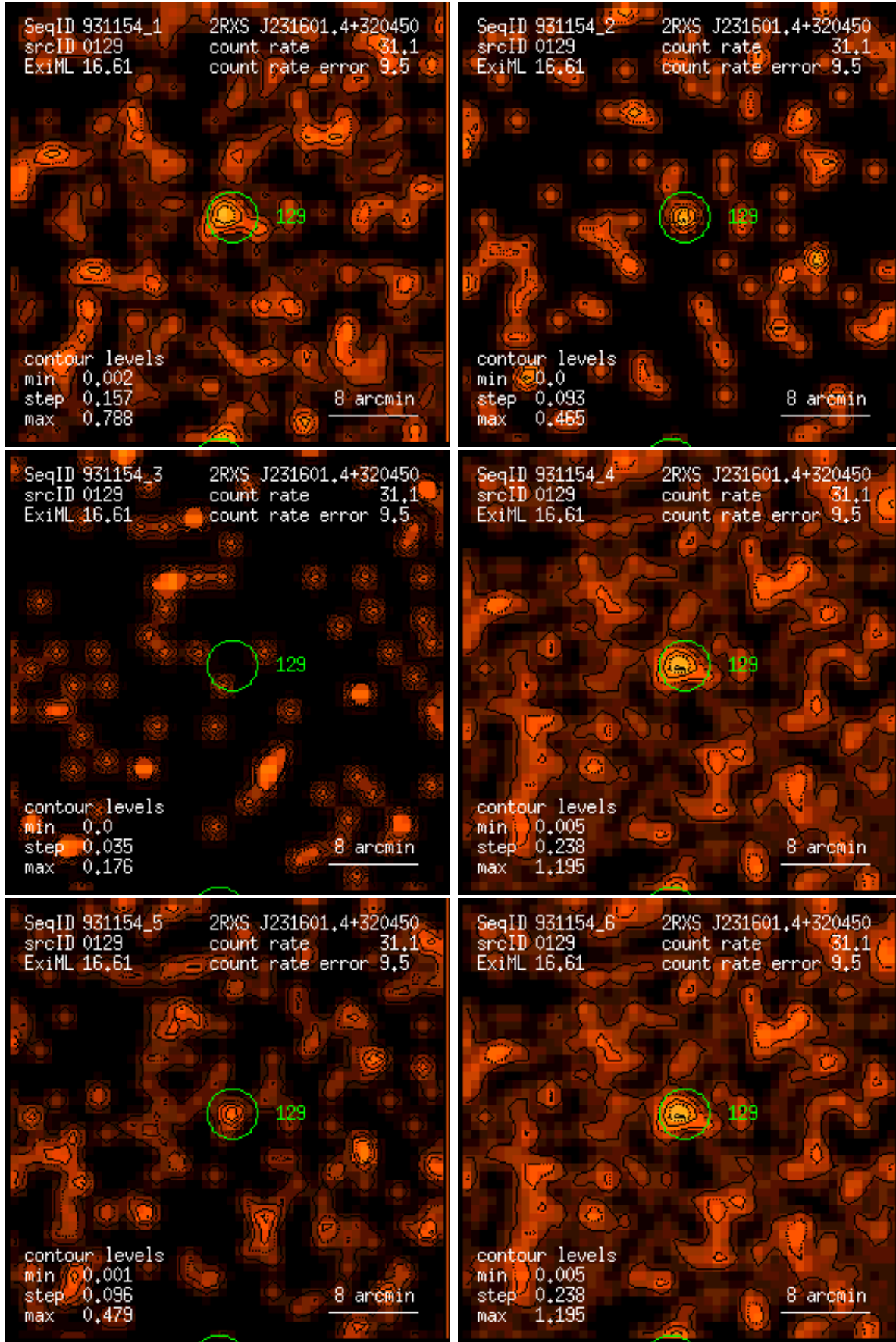
Figure 129: RASS 931154: detection 0129: band rate images, Gaussian filter: (1) PSPC channels 11 – 41, (2) 52 – 90, (3) 91 – 201, (4) 11 – 235, (5) 52 – 201, (6) 11 – 201. Broad band rates in counts/ks. Band rate contour levels in counts/ks/arcmin 2 .
