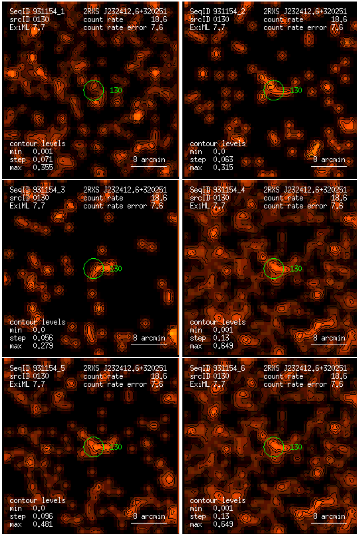
Figure 130: RASS 931154: detection 0130: band rate images, Gaussian filter: (1) PSPC channels 11 – 41, (2) 52 – 90, (3) 91 – 201, (4) 11 – 235, (5) 52 – 201, (6) 11 – 201. Broad band rates in counts/ks. Band rate contour levels in counts/ks/arcmin 2 .
