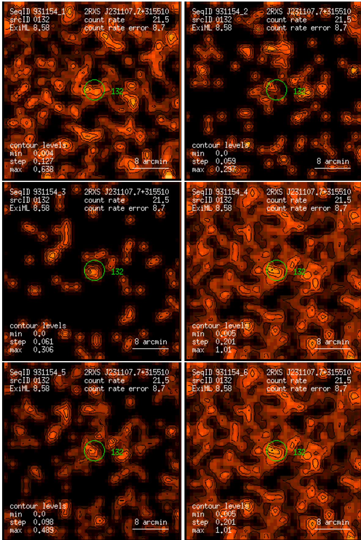
Figure 132: RASS 931154: detection 0132: band rate images, Gaussian filter: (1) PSPC channels 11 – 41, (2) 52 – 90, (3) 91 – 201, (4) 11 – 235, (5) 52 – 201, (6) 11 – 201. Broad band rates in counts/ks. Band rate contour levels in counts/ks/arcmin 2 .
