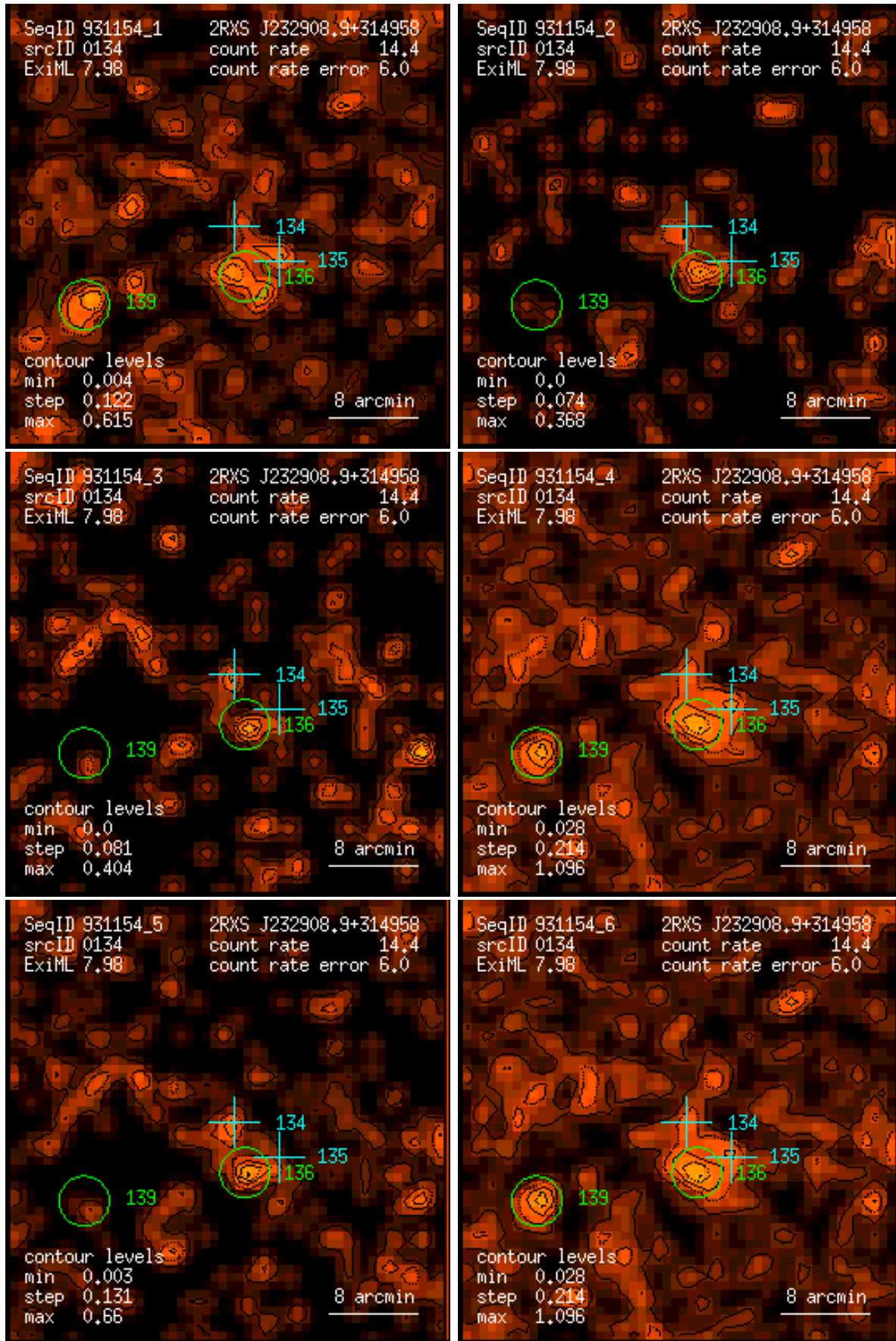
Figure 134: RASS 931154: detection 0134: band rate images, Gaussian filter: (1) PSPC channels 11 – 41, (2) 52 – 90, (3) 91 – 201, (4) 11 – 235, (5) 52 – 201, (6) 11 – 201. Broad band rates in counts/ks. Band rate contour levels in counts/ks/arcmin 2 .
